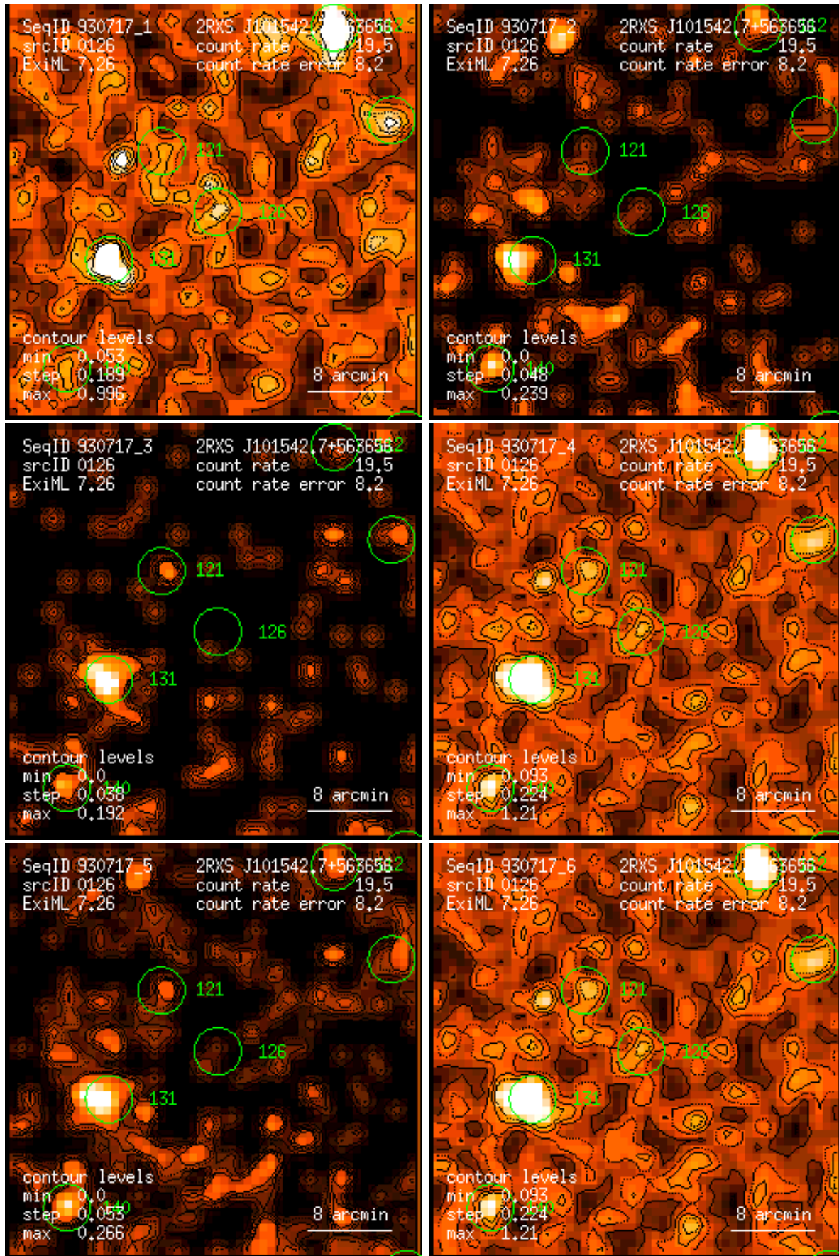
Figure 126: RASS 930717: detection 0126: band rate images, Gaussian filter: (1) PSPC channels 11 – 41, (2) 52 – 90, (3) 91 – 201, (4) 11 – 235, (5) 52 – 201, (6) 11 – 201. Broad band rates in counts/ks. Band rate contour levels in counts/ks/arcmin 2 .
