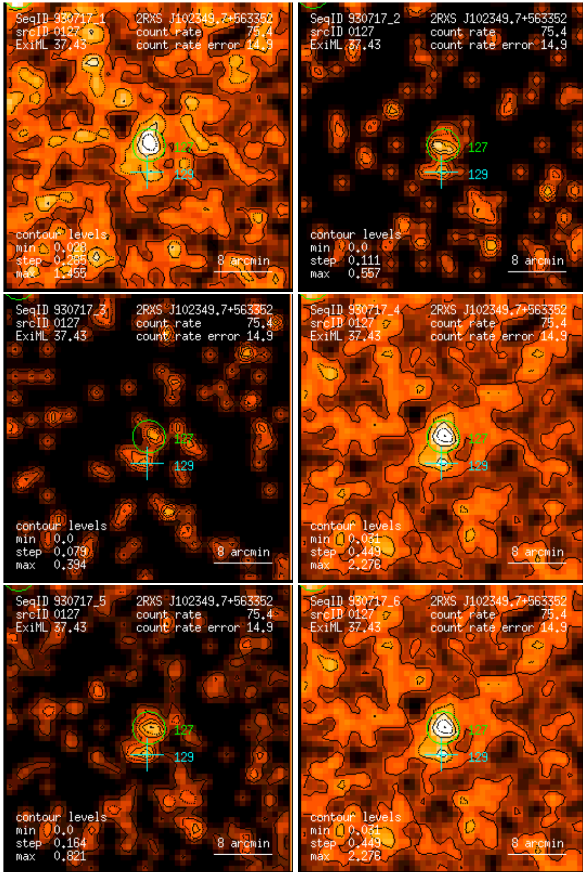
Figure 127: RASS 930717: detection 0127: band rate images, Gaussian filter: (1) PSPC channels 11 – 41, (2) 52 – 90, (3) 91 – 201, (4) 11 – 235, (5) 52 – 201, (6) 11 – 201. Broad band rates in counts/ks. Band rate contour levels in counts/ks/arcmin 2 .
