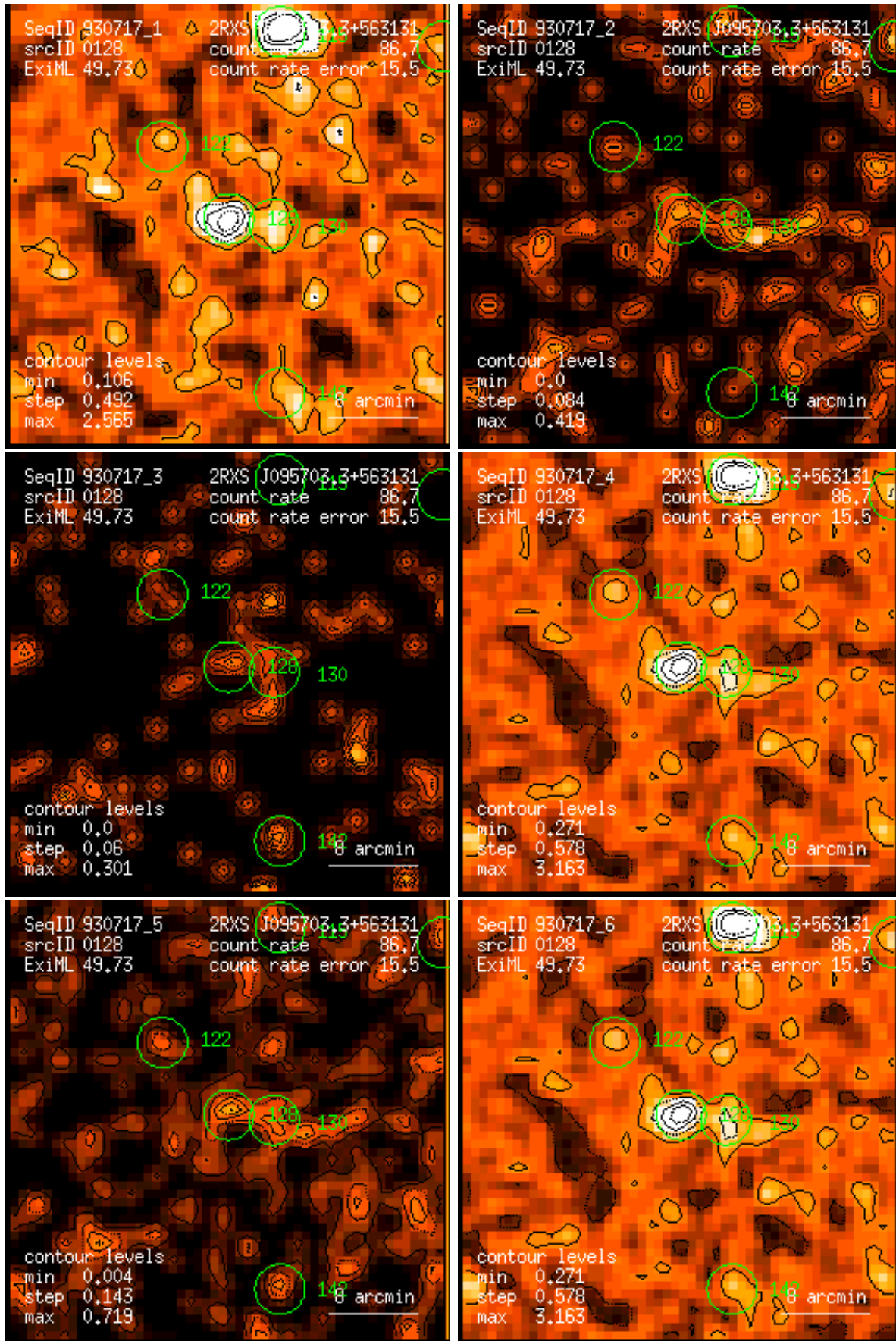
Figure 128: RASS 930717: detection 0128: band rate images, Gaussian filter: (1) PSPC channels 11 – 41, (2) 52 – 90, (3) 91 – 201, (4) 11 – 235, (5) 52 – 201, (6) 11 – 201. Broad band rates in counts/ks. Band rate contour levels in counts/ks/arcmin 2 .
