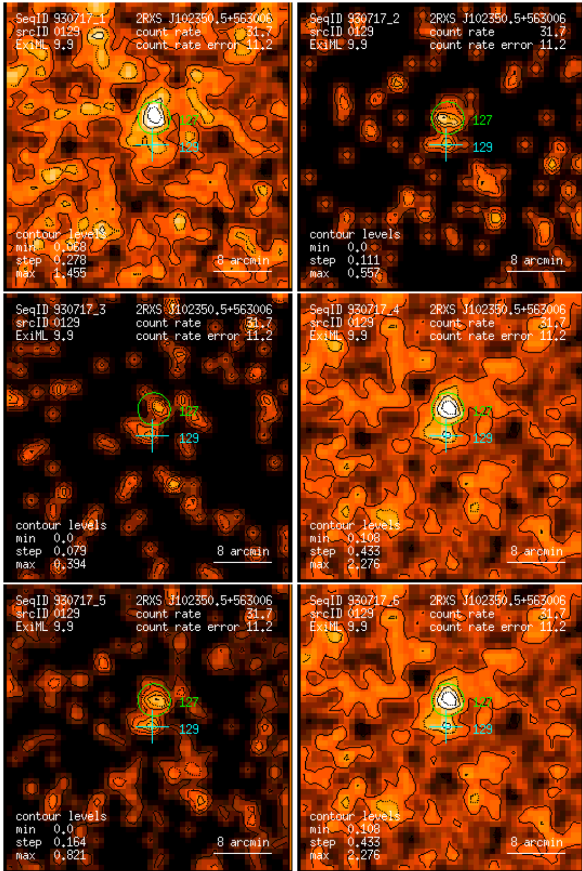
Figure 129: RASS 930717: detection 0129: band rate images, Gaussian filter: (1) PSPC channels 11 – 41, (2) 52 – 90, (3) 91 – 201, (4) 11 – 235, (5) 52 – 201, (6) 11 – 201. Broad band rates in counts/ks. Band rate contour levels in counts/ks/arcmin 2 .
