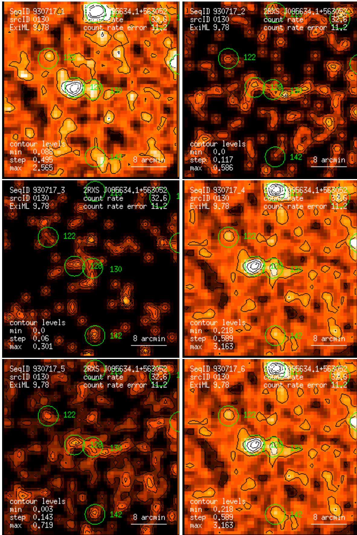
Figure 130: RASS 930717: detection 0130: band rate images, Gaussian filter: (1) PSPC channels 11 – 41, (2) 52 – 90, (3) 91 – 201, (4) 11 – 235, (5) 52 – 201, (6) 11 – 201. Broad band rates in counts/ks. Band rate contour levels in counts/ks/arcmin 2 .
