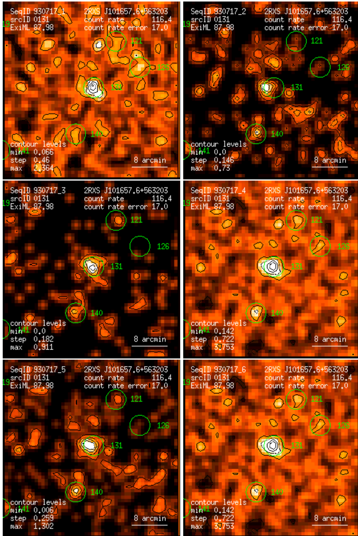
Figure 131: RASS 930717: detection 0131: band rate images, Gaussian filter: (1) PSPC channels 11 – 41, (2) 52 – 90, (3) 91 – 201, (4) 11 – 235, (5) 52 – 201, (6) 11 – 201. Broad band rates in counts/ks. Band rate contour levels in counts/ks/arcmin 2 .
