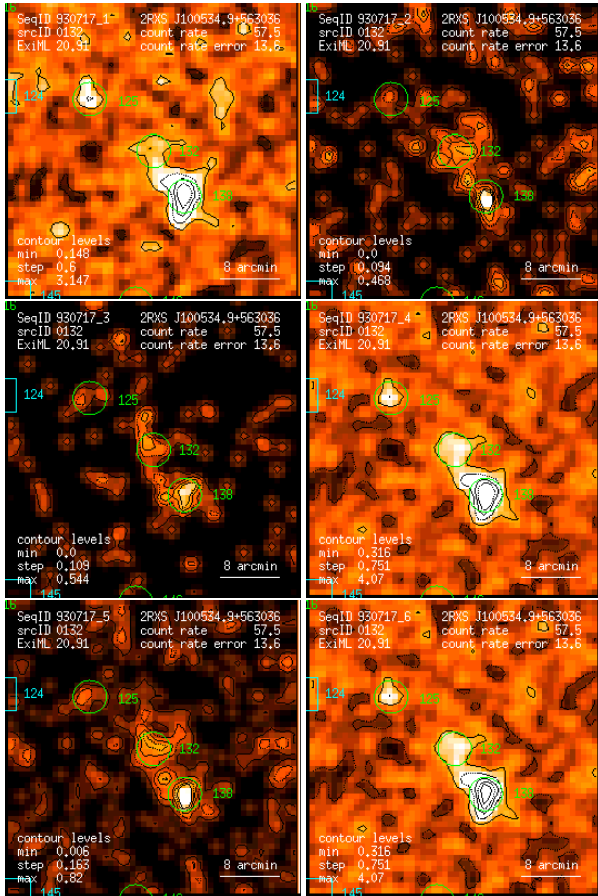
Figure 132: RASS 930717: detection 0132: band rate images, Gaussian filter: (1) PSPC channels 11 – 41, (2) 52 – 90, (3) 91 – 201, (4) 11 – 235, (5) 52 – 201, (6) 11 – 201. Broad band rates in counts/ks. Band rate contour levels in counts/ks/arcmin 2 .
