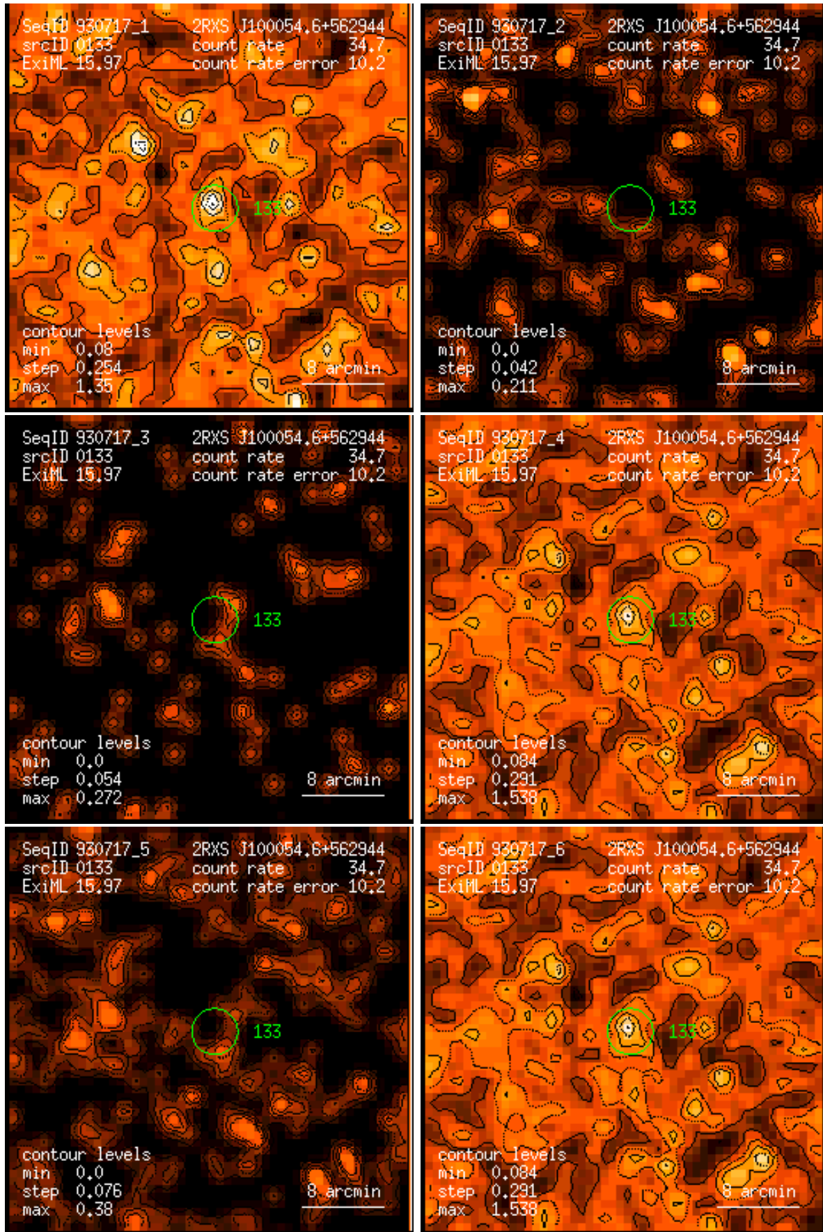
Figure 133: RASS 930717: detection 0133: band rate images, Gaussian filter: (1) PSPC channels 11 – 41, (2) 52 – 90, (3) 91 – 201, (4) 11 – 235, (5) 52 – 201, (6) 11 – 201. Broad band rates in counts/ks. Band rate contour levels in counts/ks/arcmin 2 .
