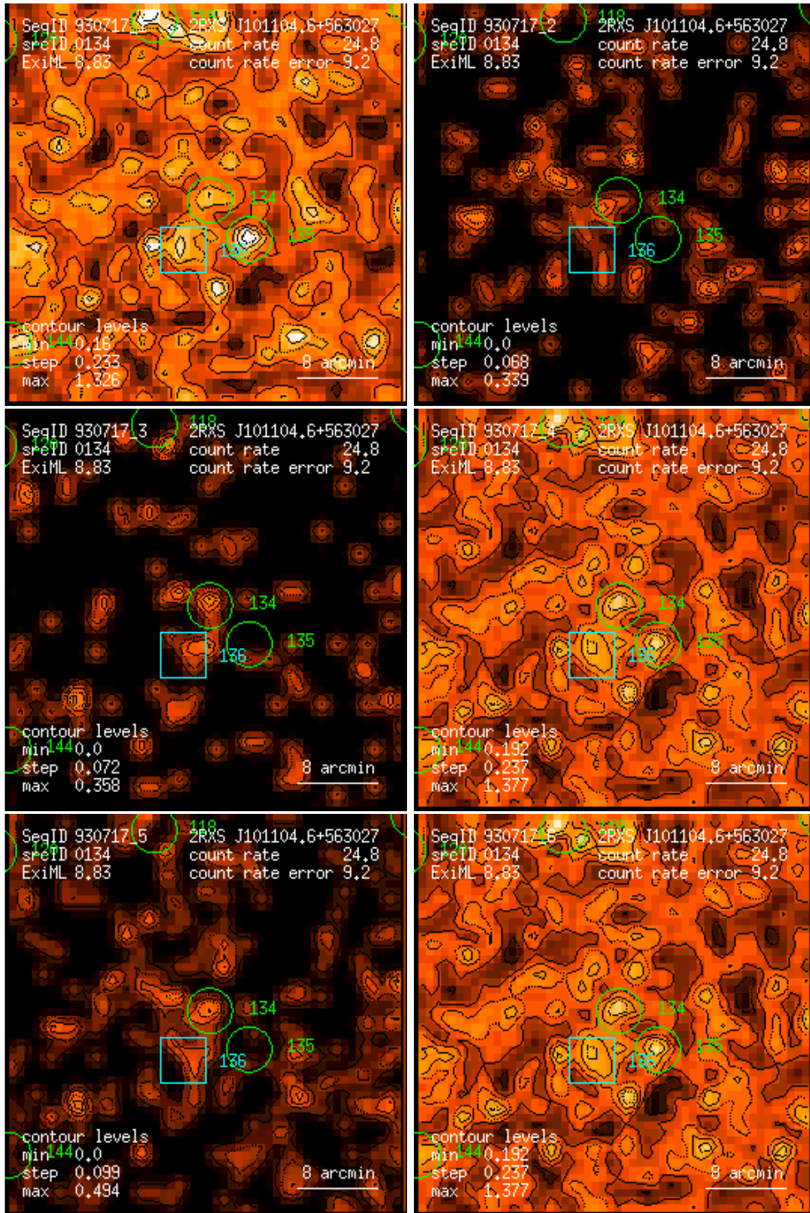
Figure 134: RASS 930717: detection 0134: band rate images, Gaussian filter: (1) PSPC channels 11 – 41, (2) 52 – 90, (3) 91 – 201, (4) 11 – 235, (5) 52 – 201, (6) 11 – 201. Broad band rates in counts/ks. Band rate contour levels in counts/ks/arcmin 2 .
