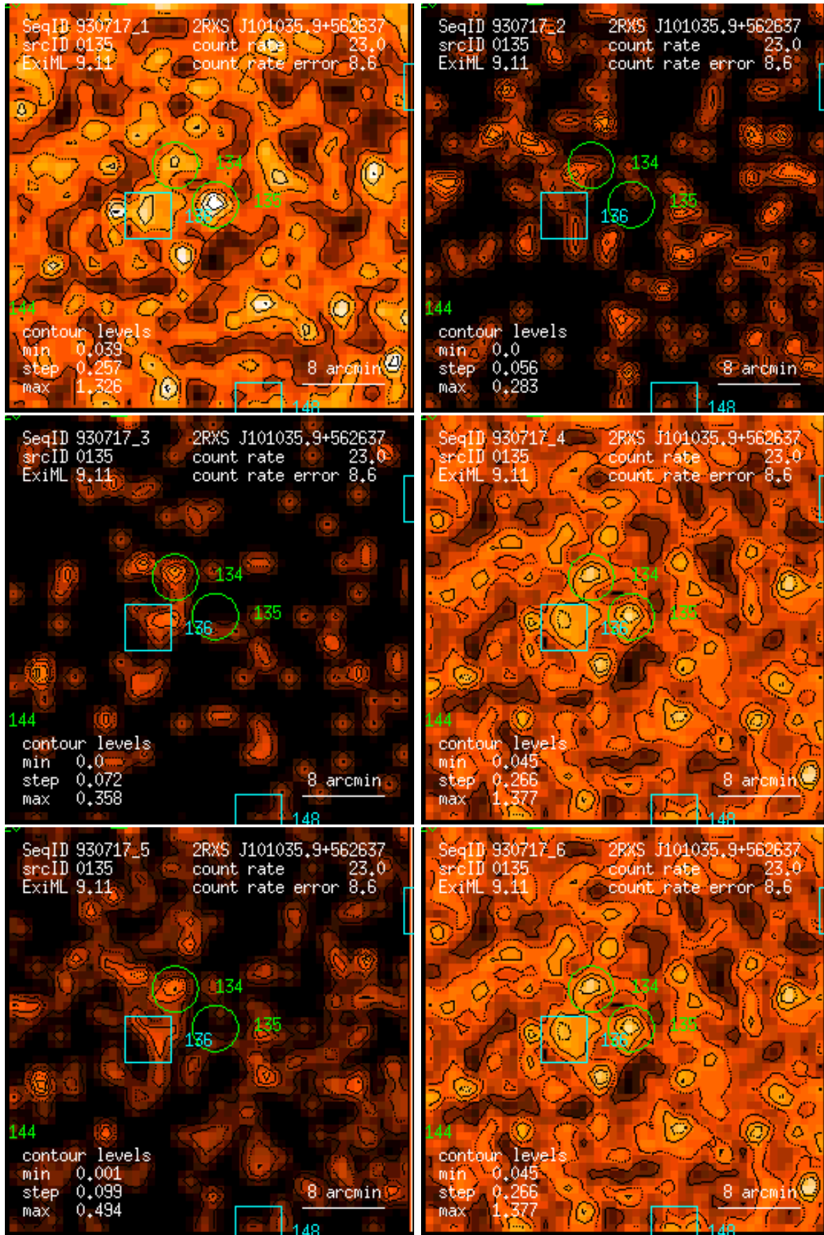
Figure 135: RASS 930717: detection 0135: band rate images, Gaussian filter: (1) PSPC channels 11 – 41, (2) 52 – 90, (3) 91 – 201, (4) 11 – 235, (5) 52 – 201, (6) 11 – 201. Broad band rates in counts/ks. Band rate contour levels in counts/ks/arcmin 2 .
