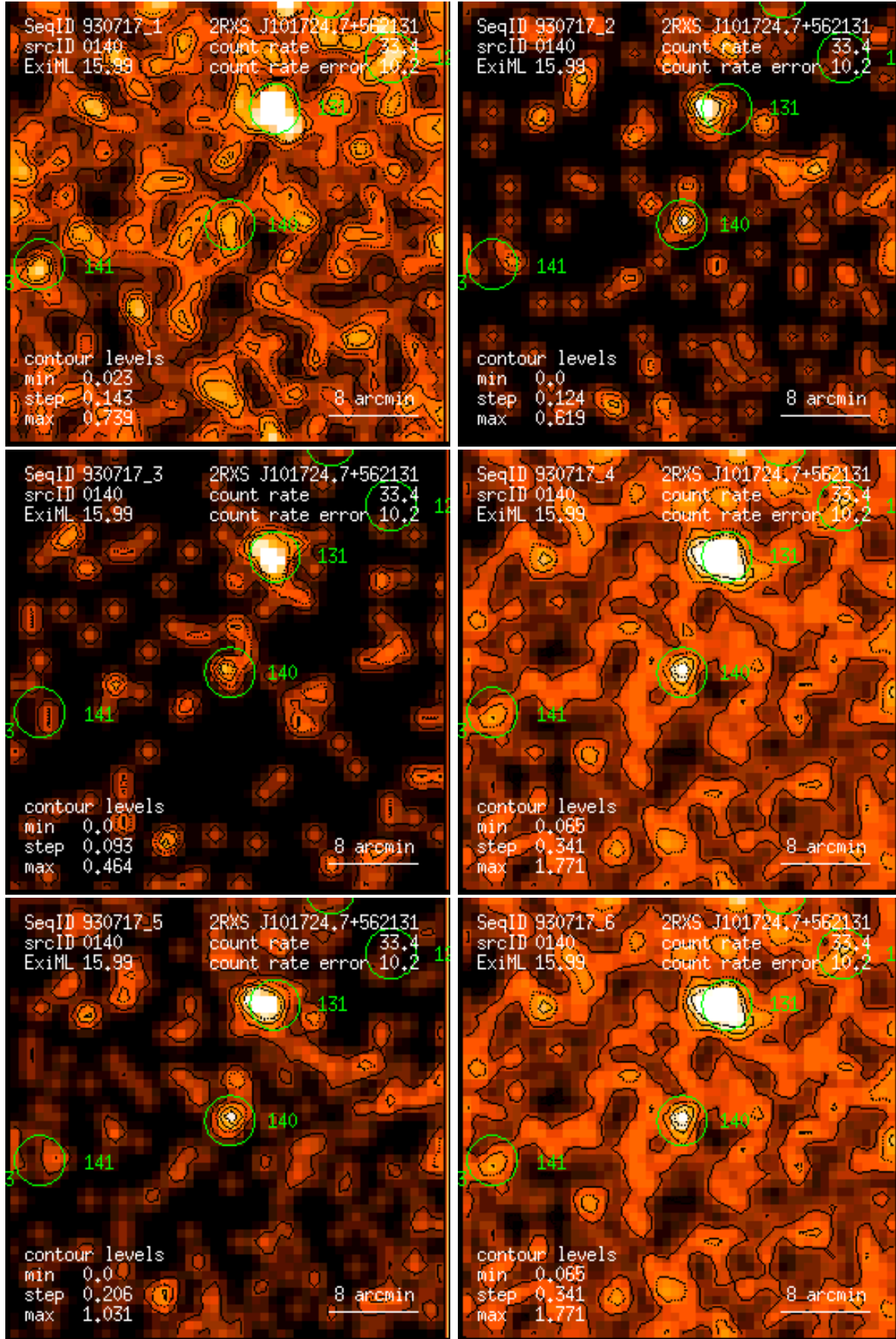
Figure 140: RASS 930717: detection 0140: band rate images, Gaussian filter: (1) PSPC channels 11 – 41, (2) 52 – 90, (3) 91 – 201, (4) 11 – 235, (5) 52 – 201, (6) 11 – 201. Broad band rates in counts/ks. Band rate contour levels in counts/ks/arcmin 2 .
