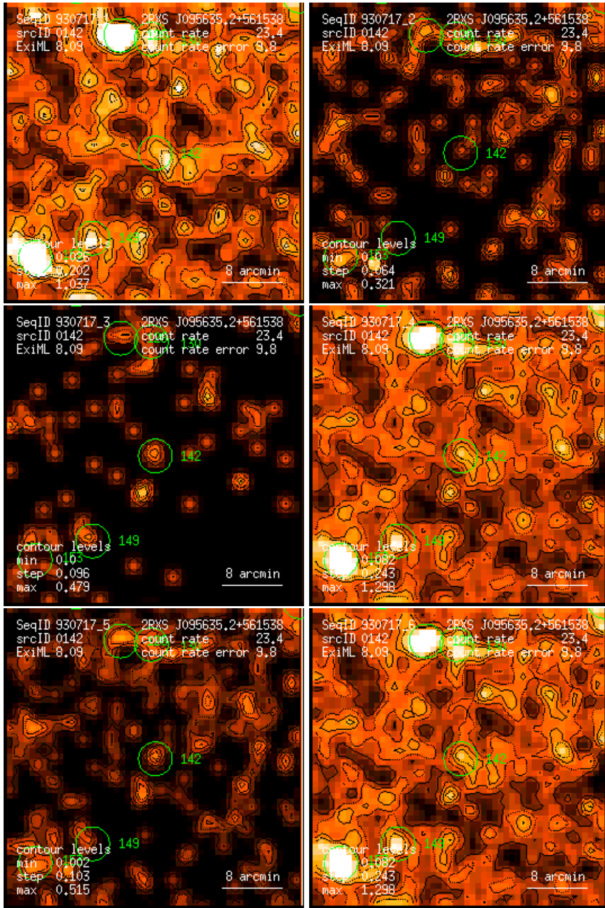
Figure 142: RASS 930717: detection 0142: band rate images, Gaussian filter: (1) PSPC channels 11 – 41, (2) 52 – 90, (3) 91 – 201, (4) 11 – 235, (5) 52 – 201, (6) 11 – 201. Broad band rates in counts/ks. Band rate contour levels in counts/ks/arcmin 2 .
