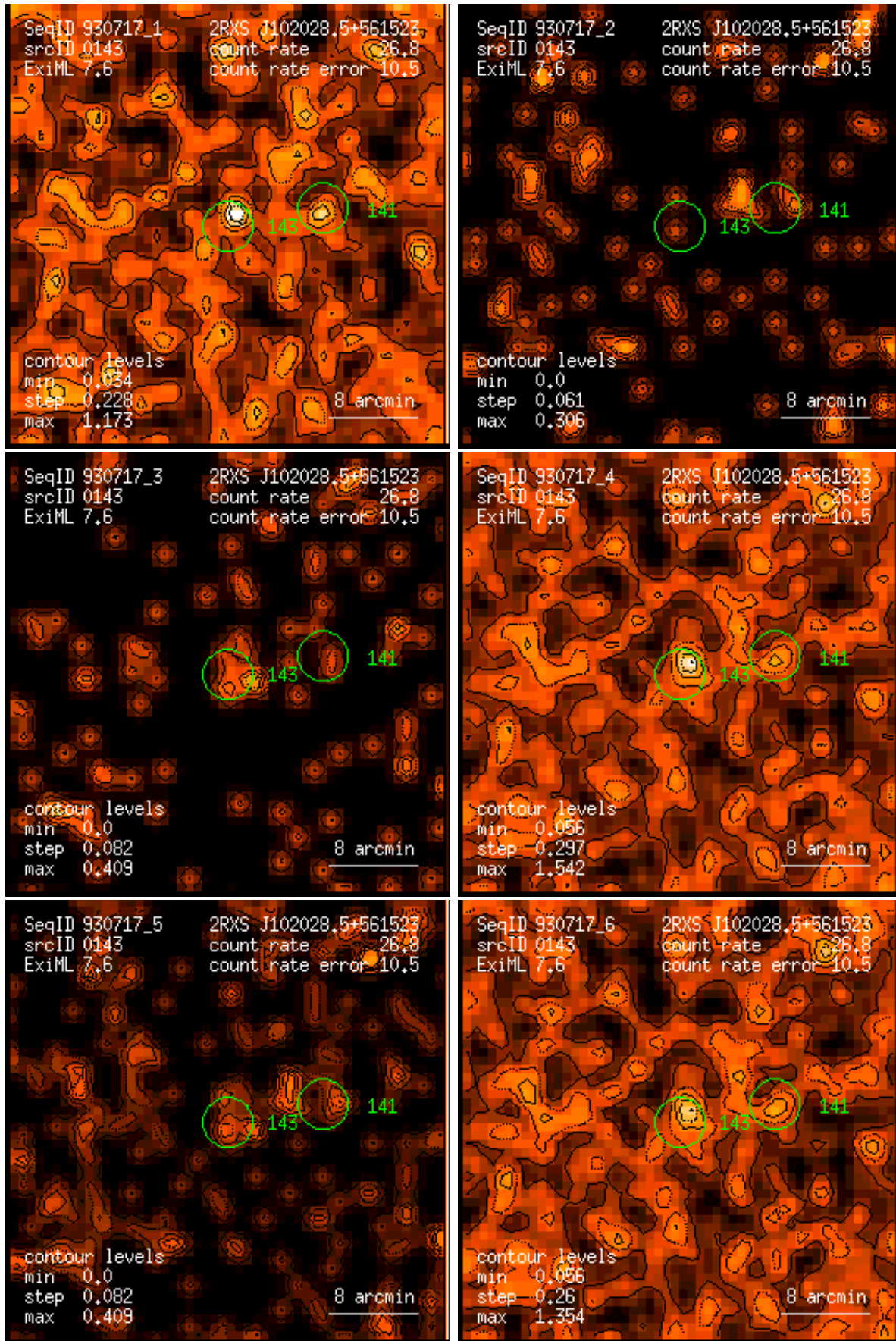
Figure 143: RASS 930717: detection 0143: band rate images, Gaussian filter: (1) PSPC channels 11 – 41, (2) 52 – 90, (3) 91 – 201, (4) 11 – 235, (5) 52 – 201, (6) 11 – 201. Broad band rates in counts/ks. Band rate contour levels in counts/ks/arcmin 2 .
