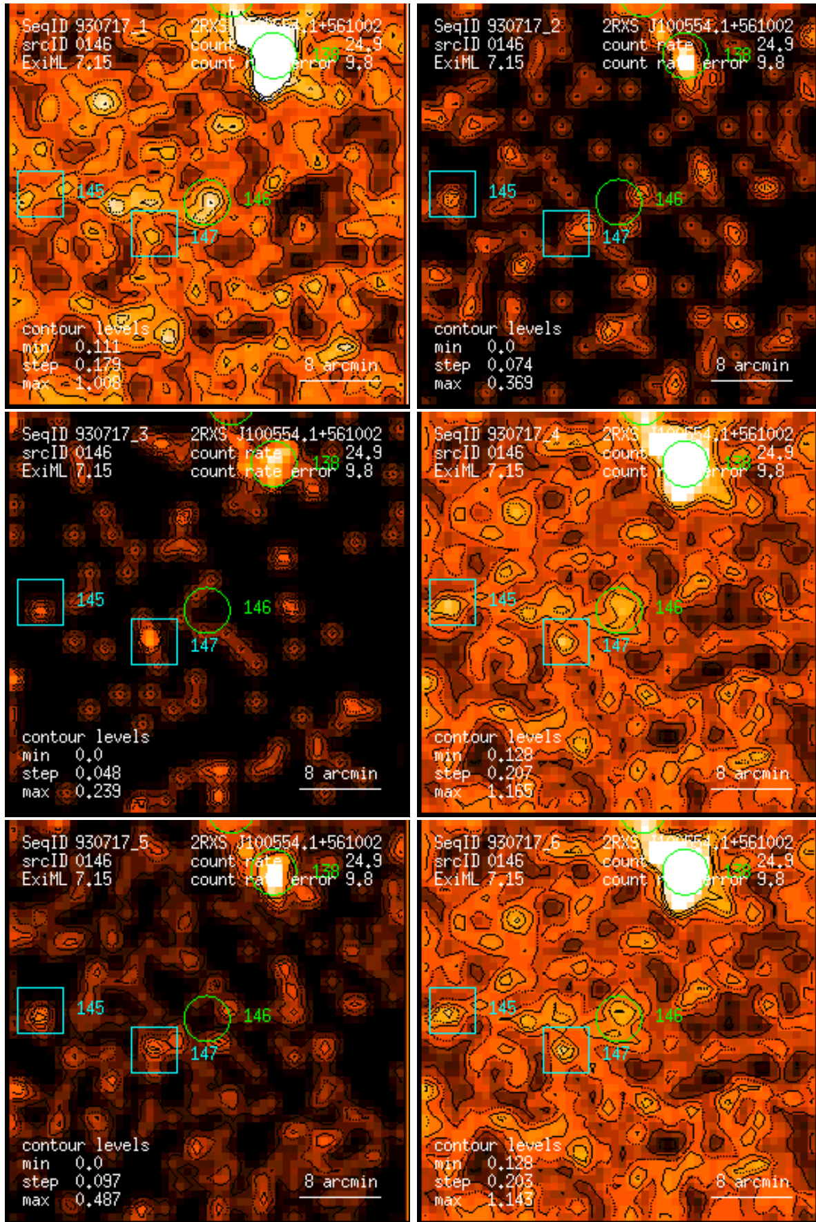
Figure 146: RASS 930717: detection 0146: band rate images, Gaussian filter: (1) PSPC channels 11 – 41, (2) 52 – 90, (3) 91 – 201, (4) 11 – 235, (5) 52 – 201, (6) 11 – 201. Broad band rates in counts/ks. Band rate contour levels in counts/ks/arcmin 2 .
