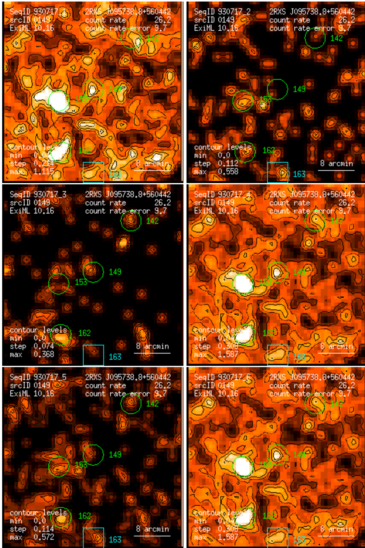
Figure 149: RASS 930717: detection 0149: band rate images, Gaussian filter: (1) PSPC channels 11 – 41, (2) 52 – 90, (3) 91 – 201, (4) 11 – 235, (5) 52 – 201, (6) 11 – 201. Broad band rates in counts/ks. Band rate contour levels in counts/ks/arcmin 2 .
