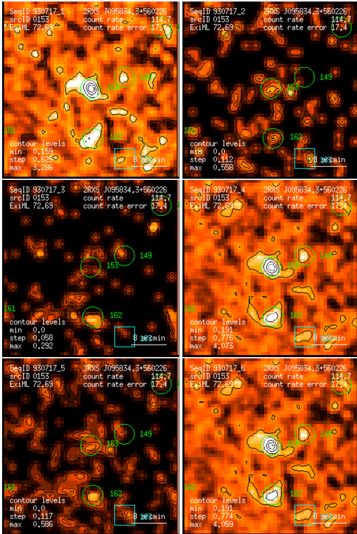
Figure 153: RASS 930717: detection 0153: band rate images, Gaussian filter: (1) PSPC channels 11 – 41, (2) 52 – 90, (3) 91 – 201, (4) 11 – 235, (5) 52 – 201, (6) 11 – 201. Broad band rates in counts/ks. Band rate contour levels in counts/ks/arcmin 2 .
