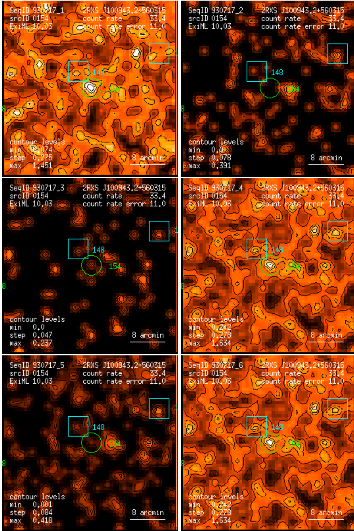
Figure 154: RASS 930717: detection 0154: band rate images, Gaussian filter: (1) PSPC channels 11 – 41, (2) 52 – 90, (3) 91 – 201, (4) 11 – 235, (5) 52 – 201, (6) 11 – 201. Broad band rates in counts/ks. Band rate contour levels in counts/ks/arcmin 2 .
