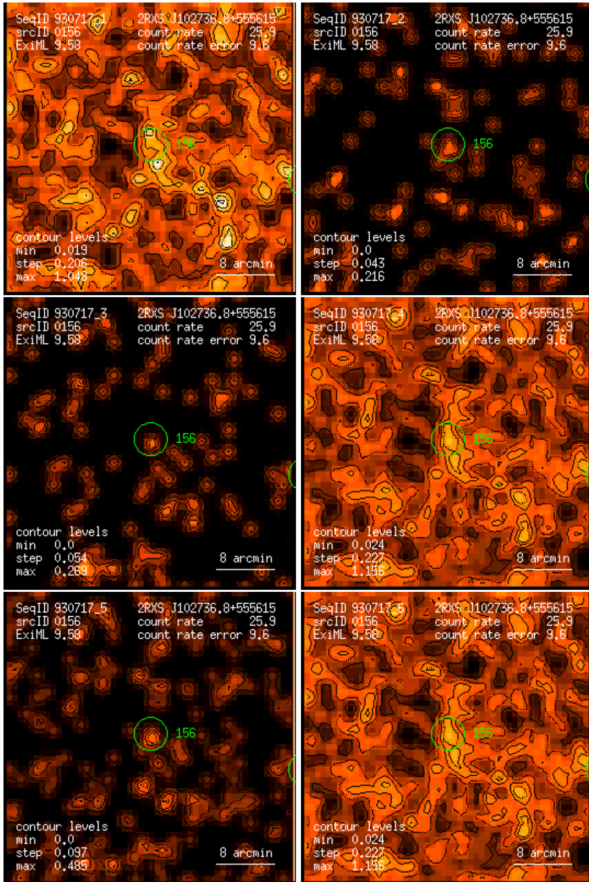
Figure 156: RASS 930717: detection 0156: band rate images, Gaussian filter: (1) PSPC channels 11 – 41, (2) 52 – 90, (3) 91 – 201, (4) 11 – 235, (5) 52 – 201, (6) 11 – 201. Broad band rates in counts/ks. Band rate contour levels in counts/ks/arcmin 2 .
