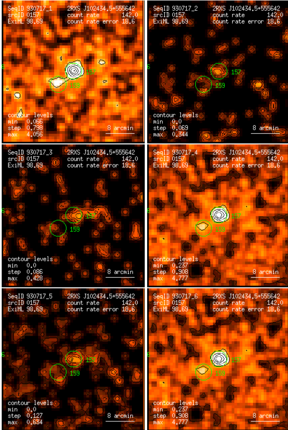
Figure 157: RASS 930717: detection 0157: band rate images, Gaussian filter: (1) PSPC channels 11 – 41, (2) 52 – 90, (3) 91 – 201, (4) 11 – 235, (5) 52 – 201, (6) 11 – 201. Broad band rates in counts/ks. Band rate contour levels in counts/ks/arcmin 2 .
