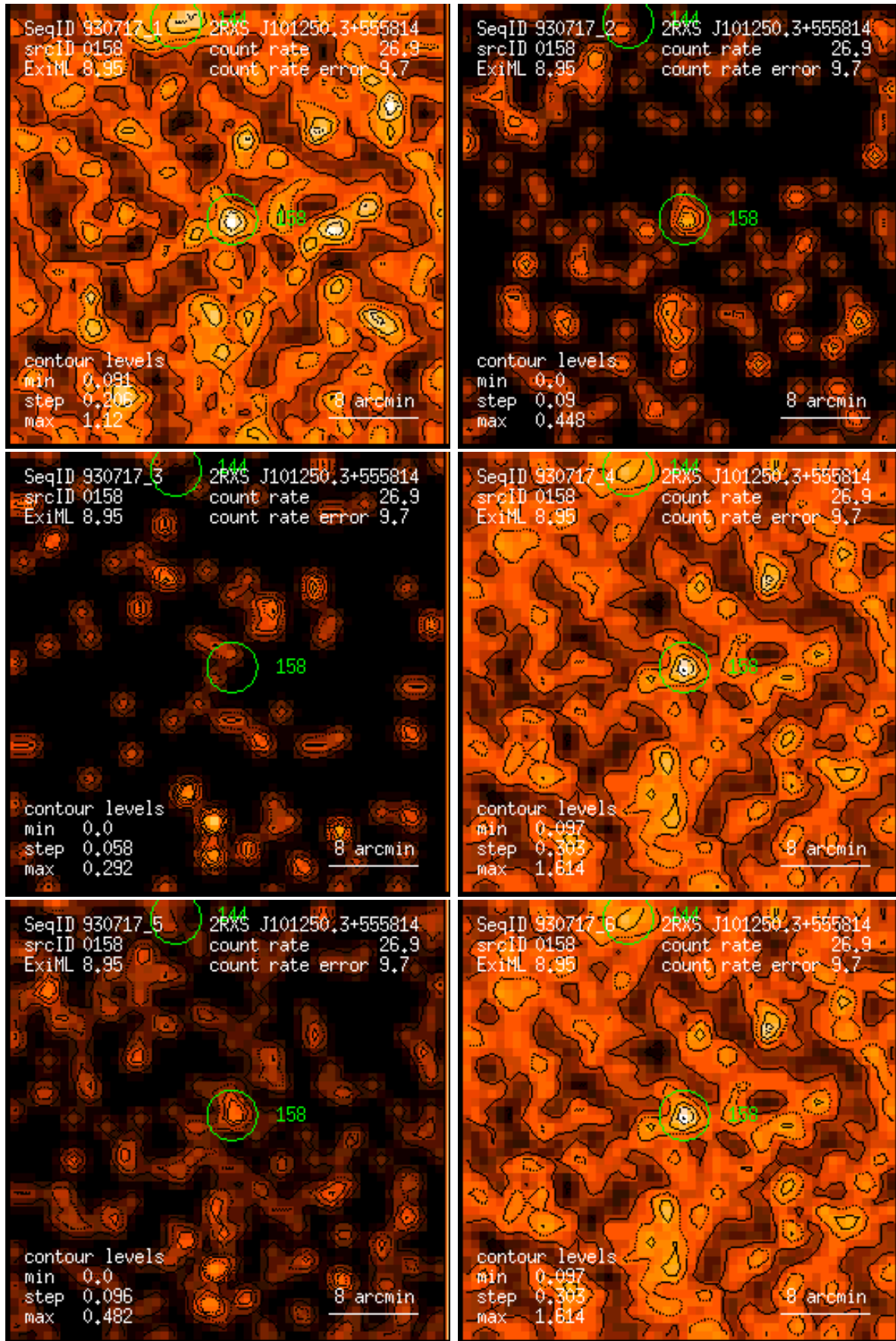
Figure 158: RASS 930717: detection 0158: band rate images, Gaussian filter: (1) PSPC channels 11 – 41, (2) 52 – 90, (3) 91 – 201, (4) 11 – 235, (5) 52 – 201, (6) 11 – 201. Broad band rates in counts/ks. Band rate contour levels in counts/ks/arcmin 2 .
