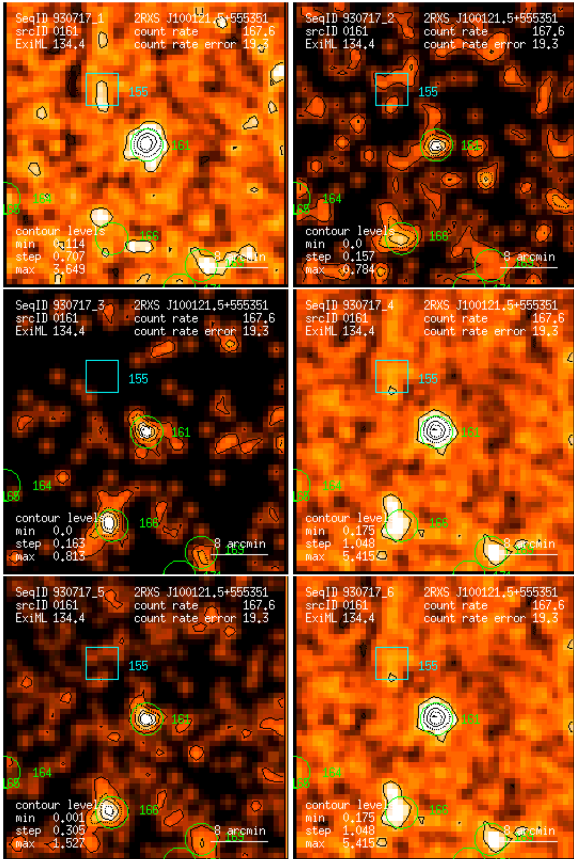
Figure 161: RASS 930717: detection 0161: band rate images, Gaussian filter: (1) PSPC channels 11 – 41, (2) 52 – 90, (3) 91 – 201, (4) 11 – 235, (5) 52 – 201, (6) 11 – 201. Broad band rates in counts/ks. Band rate contour levels in counts/ks/arcmin 2 .
