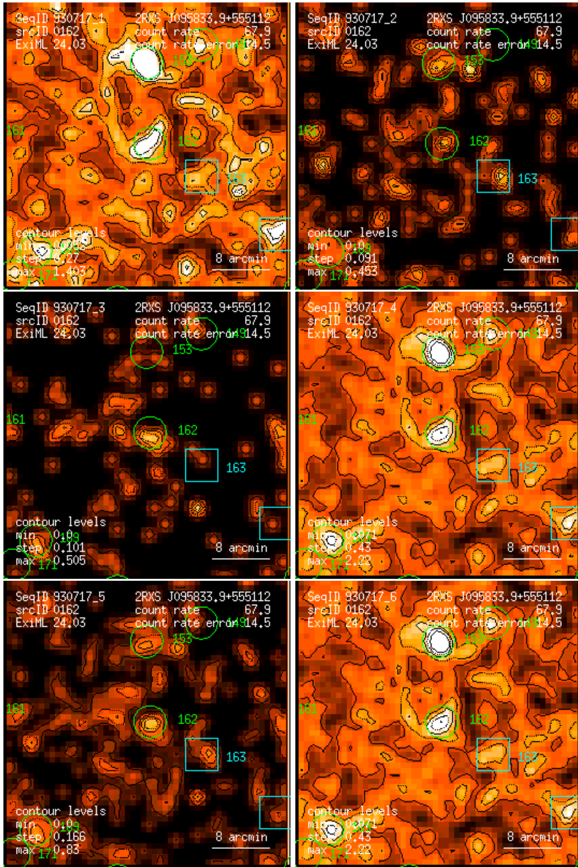
Figure 162: RASS 930717: detection 0162: band rate images, Gaussian filter: (1) PSPC channels 11 – 41, (2) 52 – 90, (3) 91 – 201, (4) 11 – 235, (5) 52 – 201, (6) 11 – 201. Broad band rates in counts/ks. Band rate contour levels in counts/ks/arcmin 2 .
