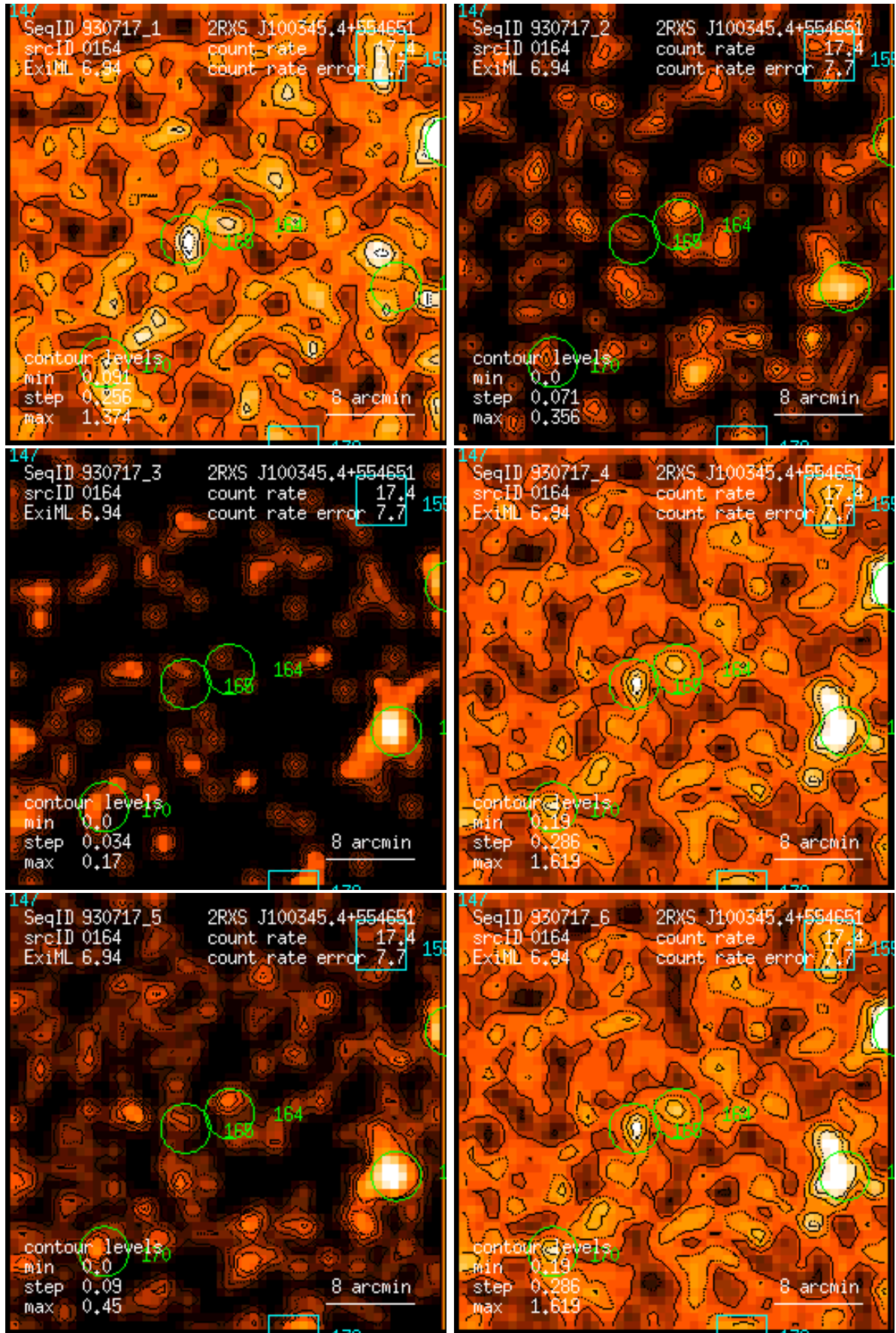
Figure 164: RASS 930717: detection 0164: band rate images, Gaussian filter: (1) PSPC channels 11 – 41, (2) 52 – 90, (3) 91 – 201, (4) 11 – 235, (5) 52 – 201, (6) 11 – 201. Broad band rates in counts/ks. Band rate contour levels in counts/ks/arcmin 2 .
