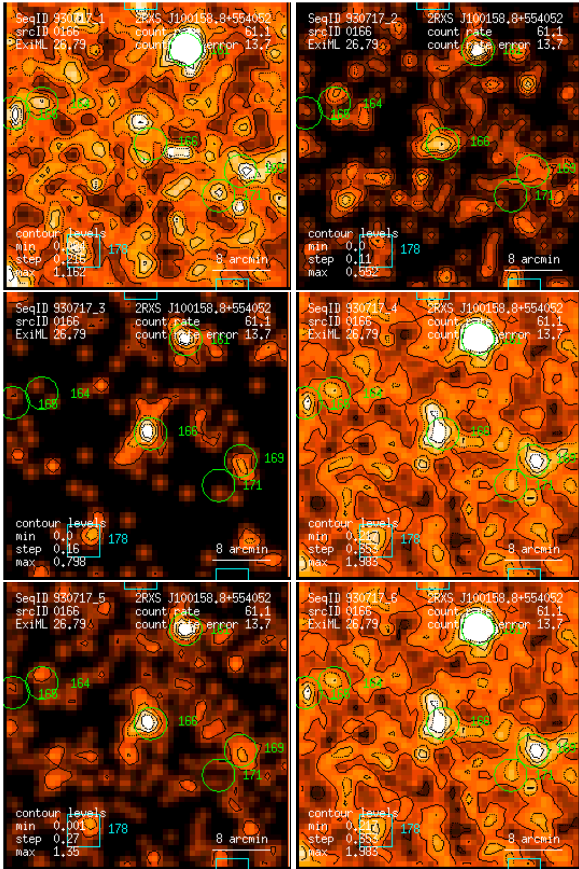
Figure 166: RASS 930717: detection 0166: band rate images, Gaussian filter: (1) PSPC channels 11 – 41, (2) 52 – 90, (3) 91 – 201, (4) 11 – 235, (5) 52 – 201, (6) 11 – 201. Broad band rates in counts/ks. Band rate contour levels in counts/ks/arcmin 2 .
