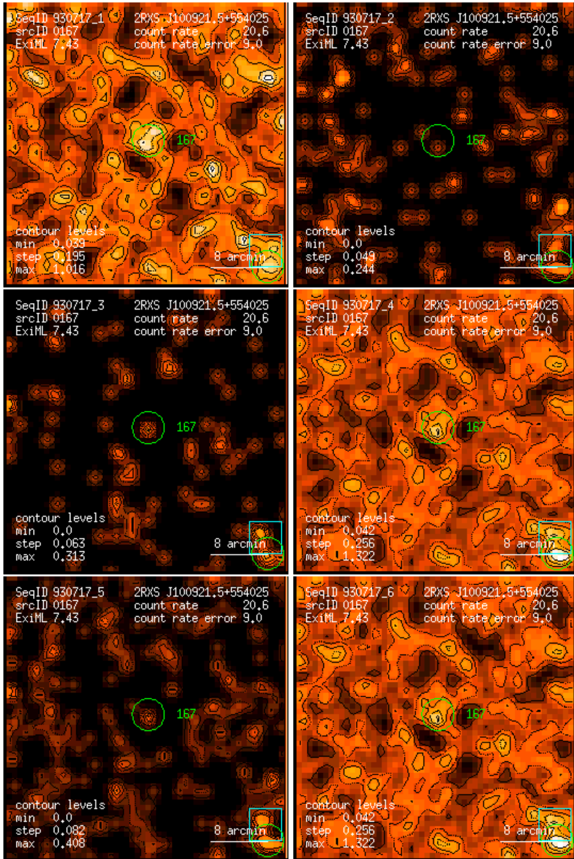
Figure 167: RASS 930717: detection 0167: band rate images, Gaussian filter: (1) PSPC channels 11 – 41, (2) 52 – 90, (3) 91 – 201, (4) 11 – 235, (5) 52 – 201, (6) 11 – 201. Broad band rates in counts/ks. Band rate contour levels in counts/ks/arcmin 2 .
