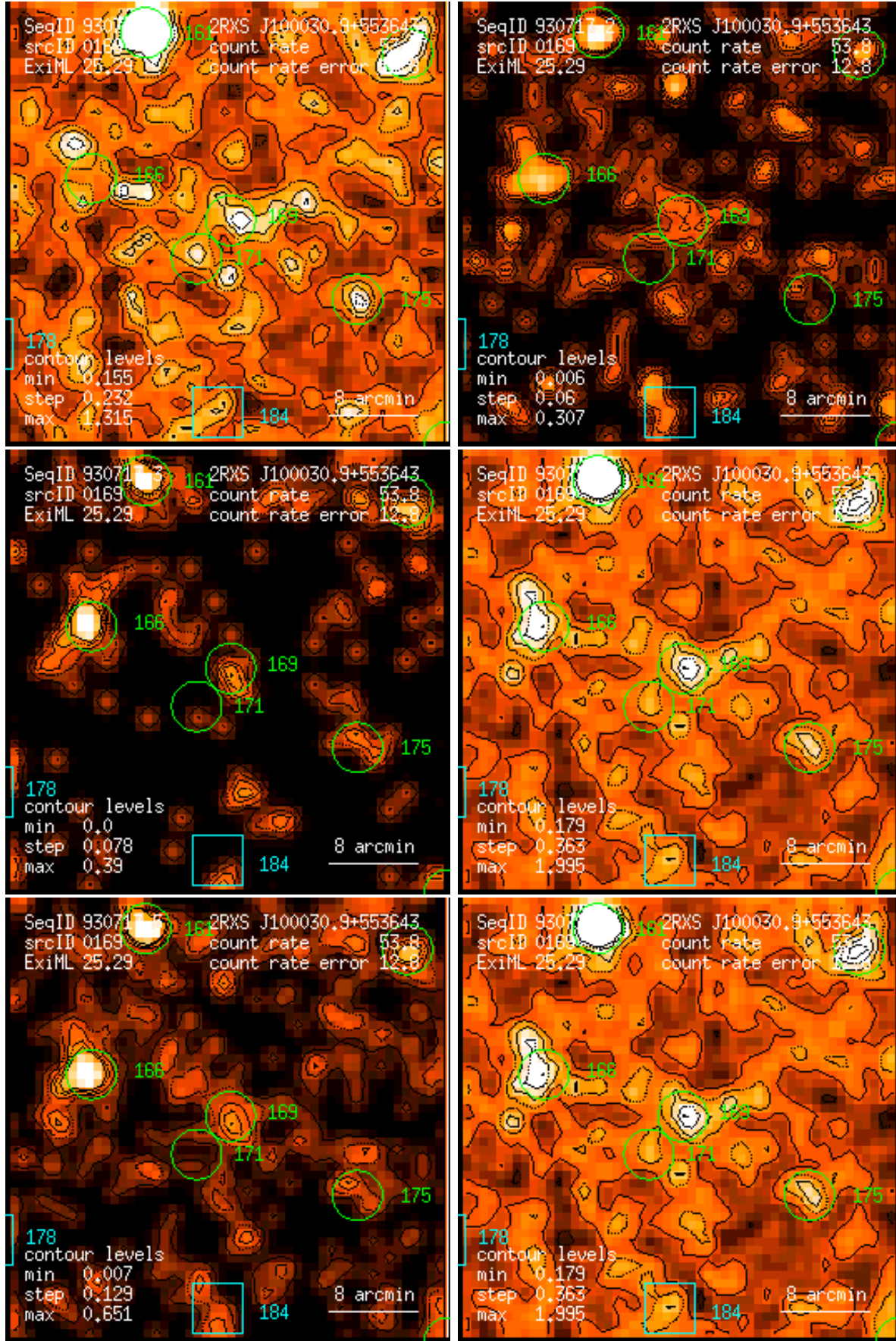
Figure 169: RASS 930717: detection 0169: band rate images, Gaussian filter: (1) PSPC channels 11 – 41, (2) 52 – 90, (3) 91 – 201, (4) 11 – 235, (5) 52 – 201, (6) 11 – 201. Broad band rates in counts/ks. Band rate contour levels in counts/ks/arcmin 2 .
