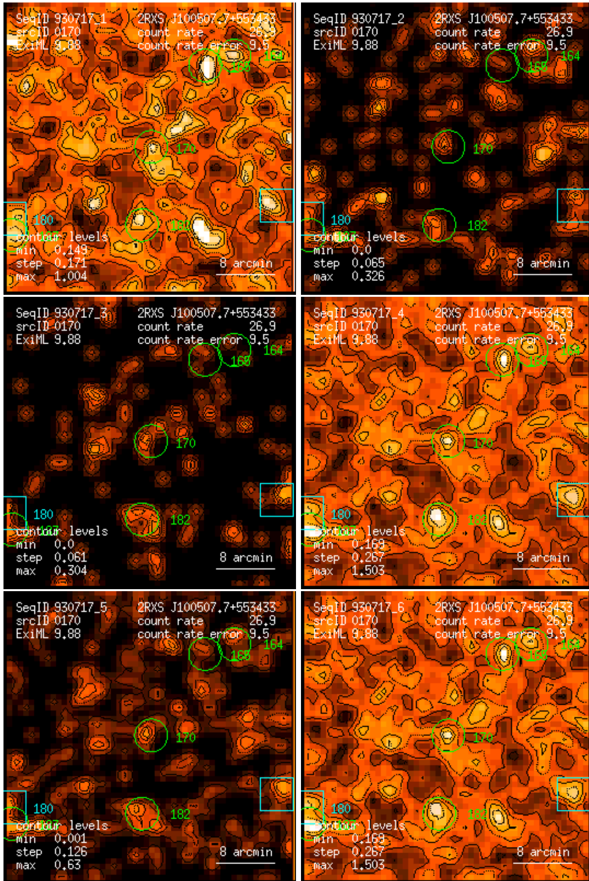
Figure 170: RASS 930717: detection 0170: band rate images, Gaussian filter: (1) PSPC channels 11 – 41, (2) 52 – 90, (3) 91 – 201, (4) 11 – 235, (5) 52 – 201, (6) 11 – 201. Broad band rates in counts/ks. Band rate contour levels in counts/ks/arcmin 2 .
