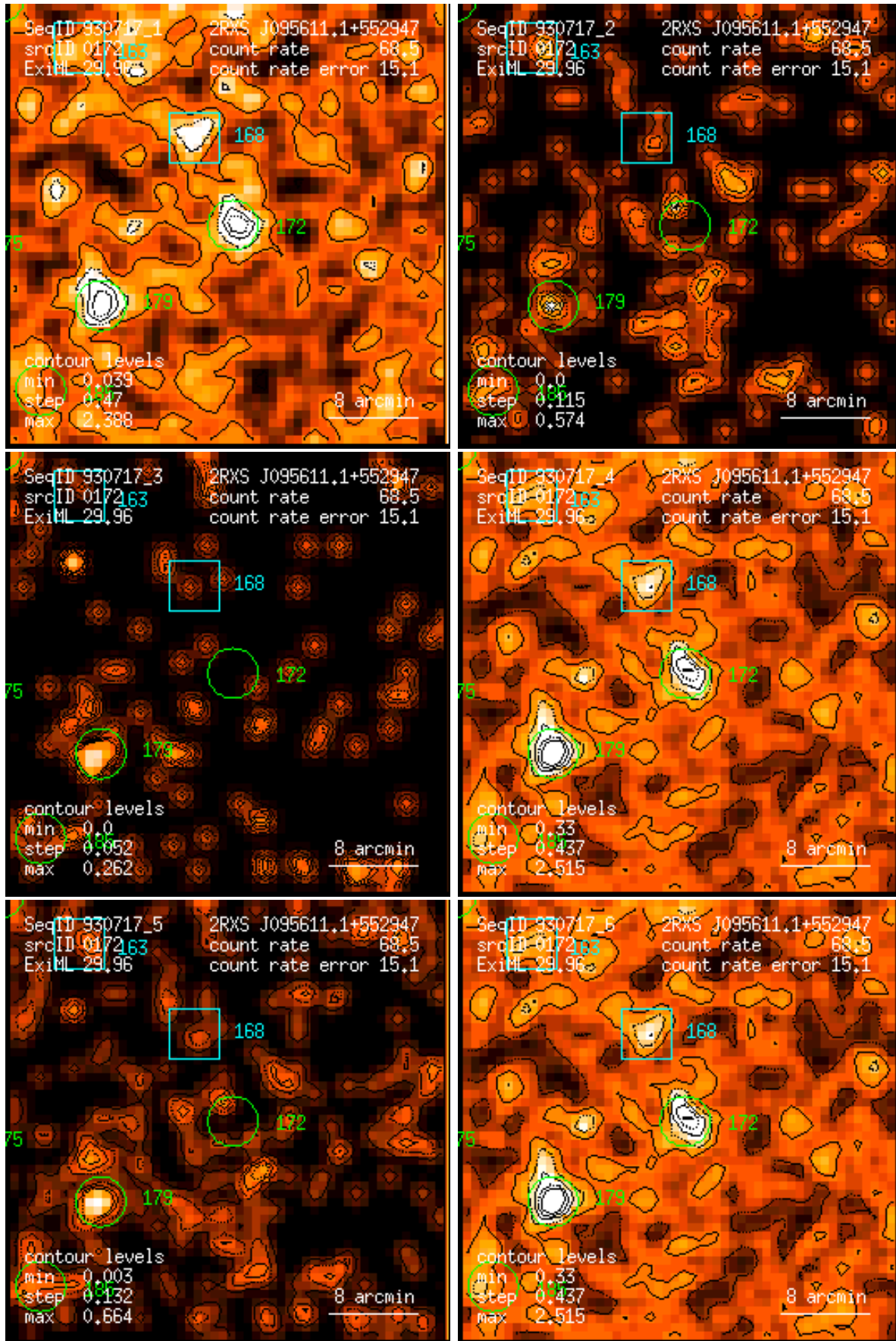
Figure 172: RASS 930717: detection 0172: band rate images, Gaussian filter: (1) PSPC channels 11 – 41, (2) 52 – 90, (3) 91 – 201, (4) 11 – 235, (5) 52 – 201, (6) 11 – 201. Broad band rates in counts/ks. Band rate contour levels in counts/ks/arcmin 2 .
