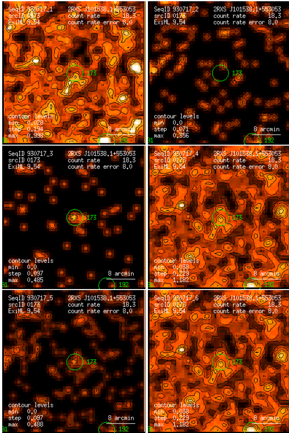
Figure 173: RASS 930717: detection 0173: band rate images, Gaussian filter: (1) PSPC channels 11 – 41, (2) 52 – 90, (3) 91 – 201, (4) 11 – 235, (5) 52 – 201, (6) 11 – 201. Broad band rates in counts/ks. Band rate contour levels in counts/ks/arcmin 2 .
