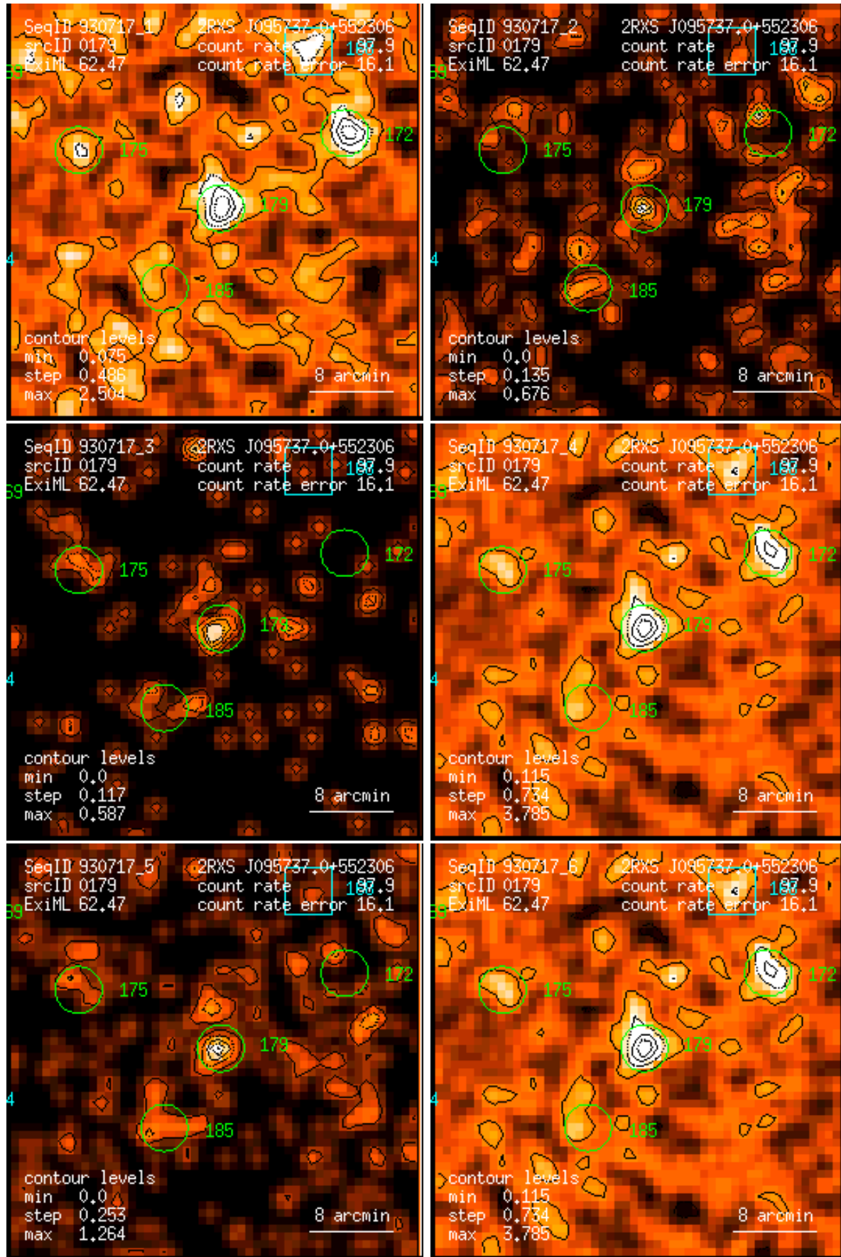
Figure 179: RASS 930717: detection 0179: band rate images, Gaussian filter: (1) PSPC channels 11 – 41, (2) 52 – 90, (3) 91 – 201, (4) 11 – 235, (5) 52 – 201, (6) 11 – 201. Broad band rates in counts/ks. Band rate contour levels in counts/ks/arcmin 2 .
