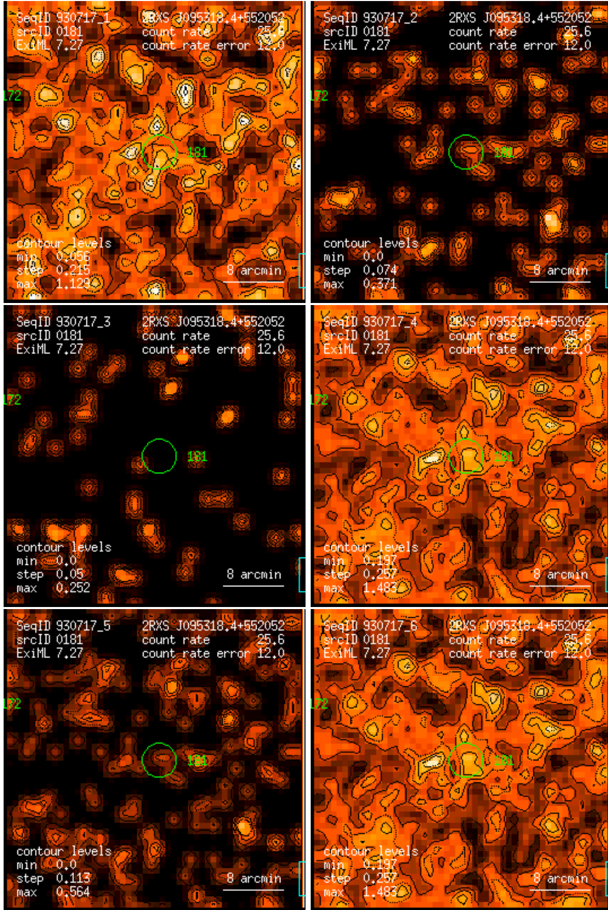
Figure 181: RASS 930717: detection 0181: band rate images, Gaussian filter: (1) PSPC channels 11 – 41, (2) 52 – 90, (3) 91 – 201, (4) 11 – 235, (5) 52 – 201, (6) 11 – 201. Broad band rates in counts/ks. Band rate contour levels in counts/ks/arcmin 2 .
