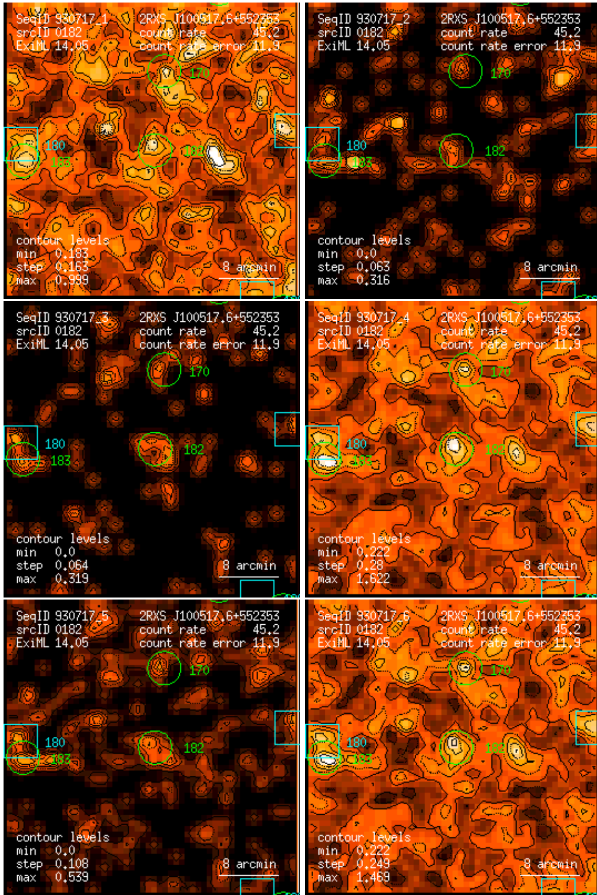
Figure 182: RASS 930717: detection 0182: band rate images, Gaussian filter: (1) PSPC channels 11 – 41, (2) 52 – 90, (3) 91 – 201, (4) 11 – 235, (5) 52 – 201, (6) 11 – 201. Broad band rates in counts/ks. Band rate contour levels in counts/ks/arcmin 2 .
