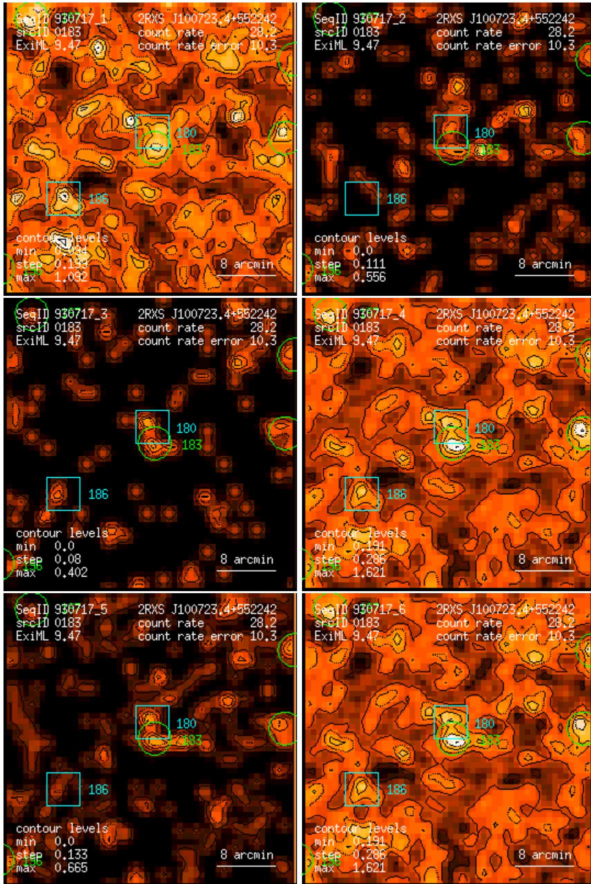
Figure 183: RASS 930717: detection 0183: band rate images, Gaussian filter: (1) PSPC channels 11 – 41, (2) 52 – 90, (3) 91 – 201, (4) 11 – 235, (5) 52 – 201, (6) 11 – 201. Broad band rates in counts/ks. Band rate contour levels in counts/ks/arcmin 2 .
