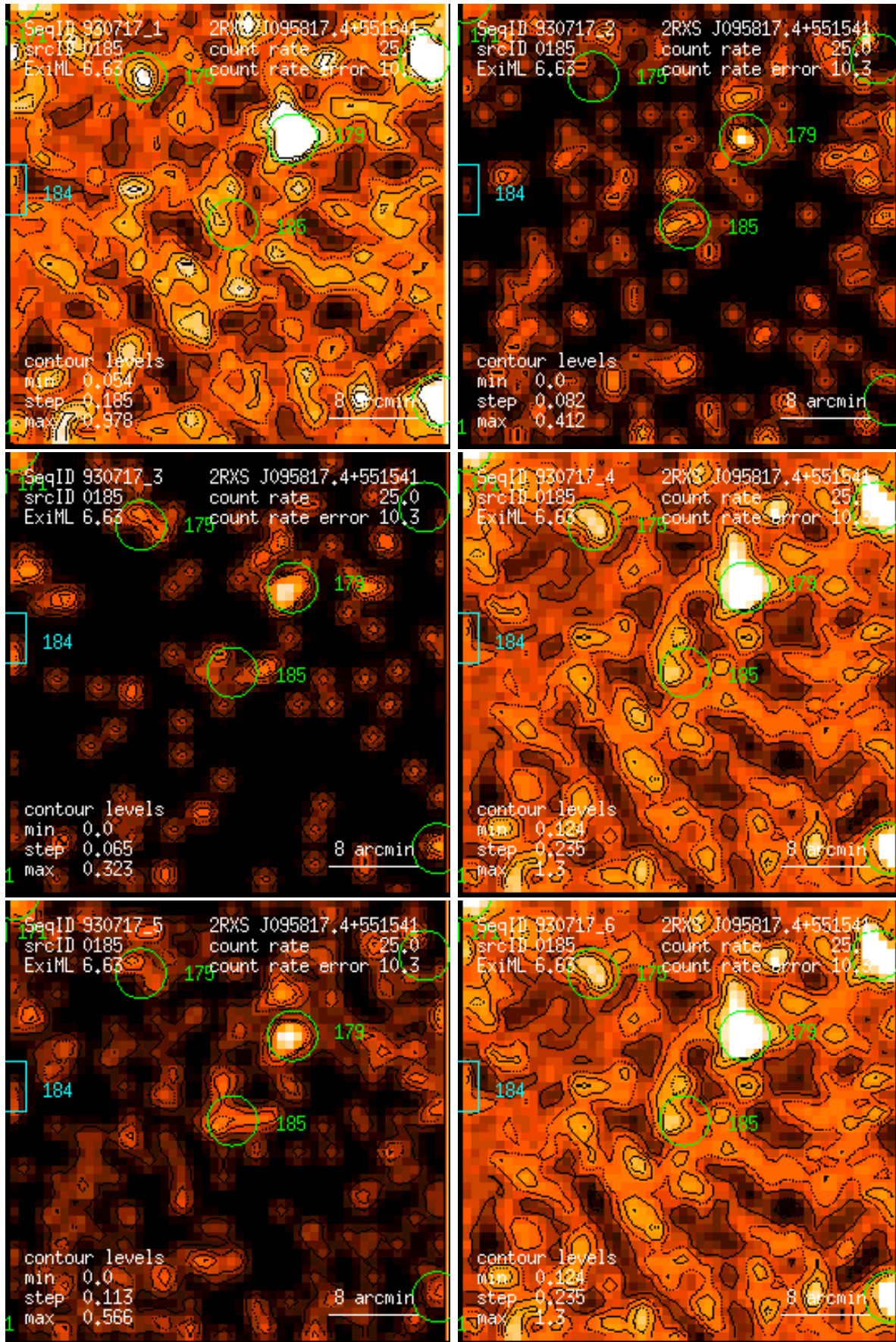
Figure 185: RASS 930717: detection 0185: band rate images, Gaussian filter: (1) PSPC channels 11 – 41, (2) 52 – 90, (3) 91 – 201, (4) 11 – 235, (5) 52 – 201, (6) 11 – 201. Broad band rates in counts/ks. Band rate contour levels in counts/ks/arcmin 2 .
