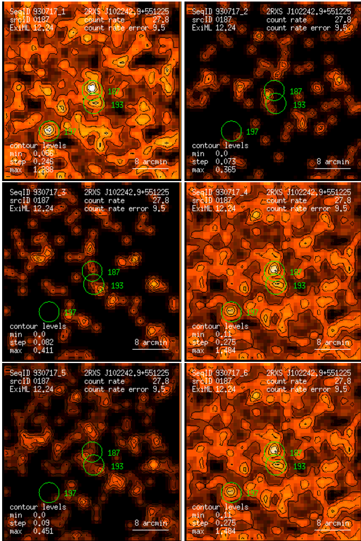
Figure 187: RASS 930717: detection 0187: band rate images, Gaussian filter: (1) PSPC channels 11 – 41, (2) 52 – 90, (3) 91 – 201, (4) 11 – 235, (5) 52 – 201, (6) 11 – 201. Broad band rates in counts/ks. Band rate contour levels in counts/ks/arcmin 2 .
