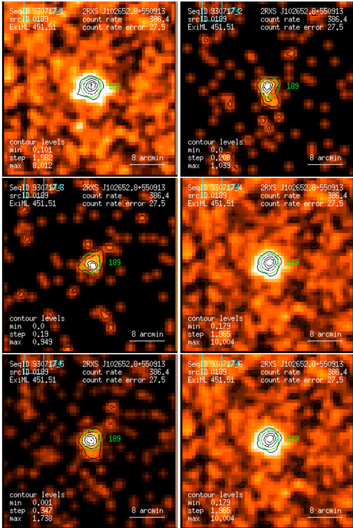
Figure 189: RASS 930717: detection 0189: band rate images, Gaussian filter: (1) PSPC channels 11 – 41, (2) 52 – 90, (3) 91 – 201, (4) 11 – 235, (5) 52 – 201, (6) 11 – 201. Broad band rates in counts/ks. Band rate contour levels in counts/ks/arcmin 2 .
