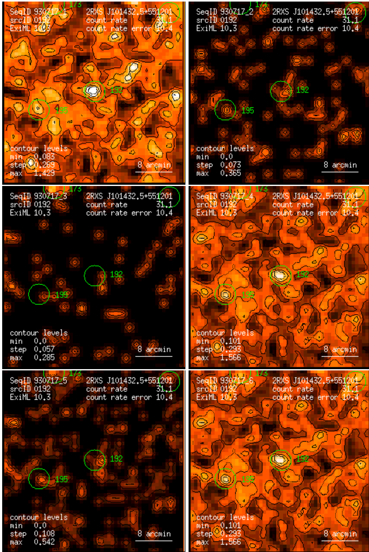
Figure 192: RASS 930717: detection 0192: band rate images, Gaussian filter: (1) PSPC channels 11 – 41, (2) 52 – 90, (3) 91 – 201, (4) 11 – 235, (5) 52 – 201, (6) 11 – 201. Broad band rates in counts/ks. Band rate contour levels in counts/ks/arcmin 2 .
