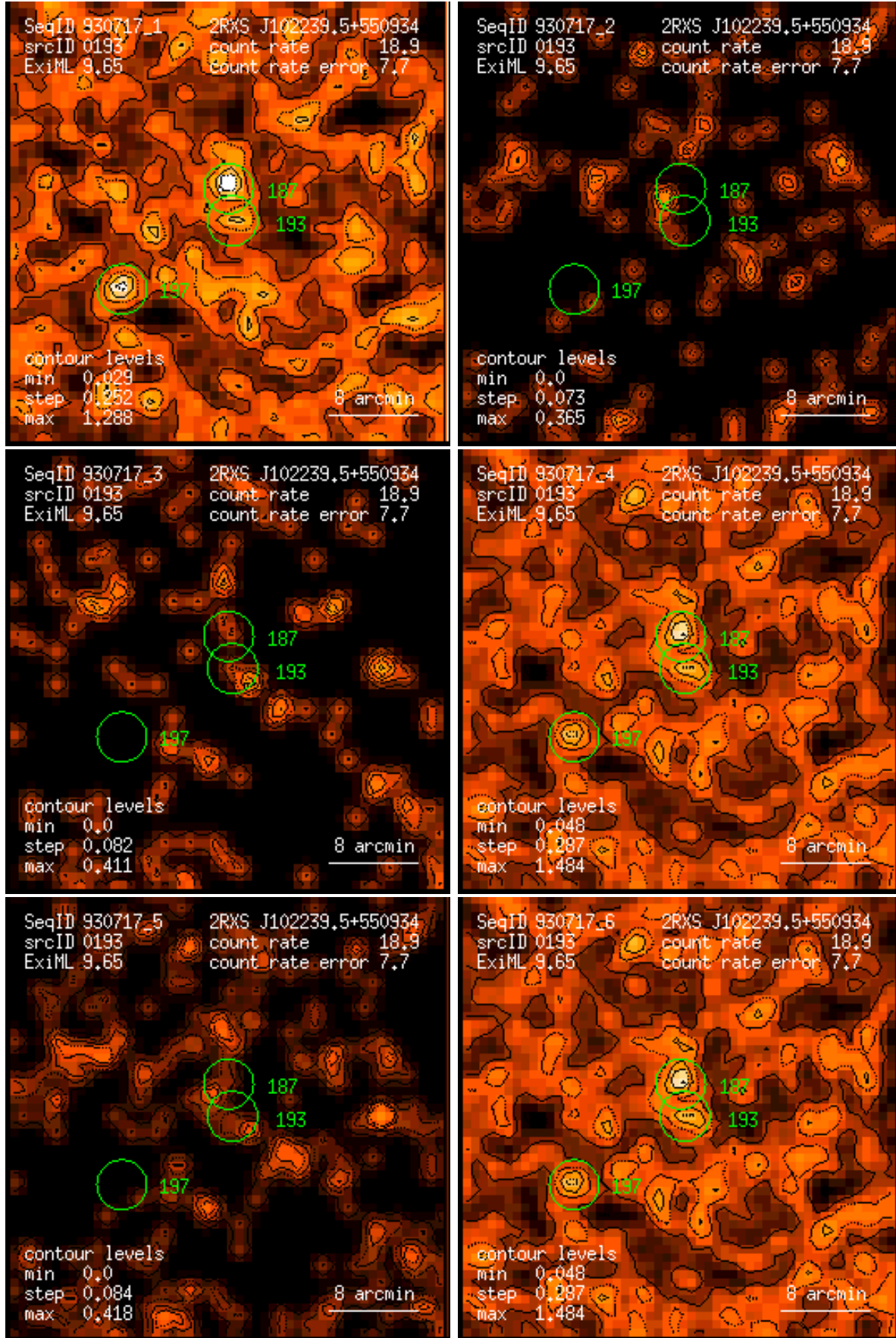
Figure 193: RASS 930717: detection 0193: band rate images, Gaussian filter: (1) PSPC channels 11 – 41, (2) 52 – 90, (3) 91 – 201, (4) 11 – 235, (5) 52 – 201, (6) 11 – 201. Broad band rates in counts/ks. Band rate contour levels in counts/ks/arcmin 2 .
