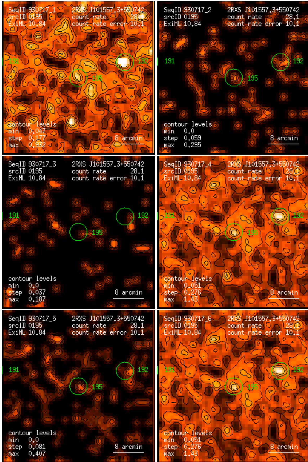
Figure 195: RASS 930717: detection 0195: band rate images, Gaussian filter: (1) PSPC channels 11 – 41, (2) 52 – 90, (3) 91 – 201, (4) 11 – 235, (5) 52 – 201, (6) 11 – 201. Broad band rates in counts/ks. Band rate contour levels in counts/ks/arcmin 2 .
