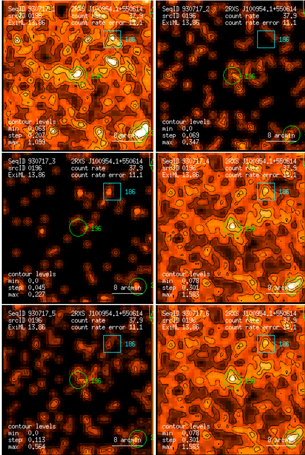
Figure 196: RASS 930717: detection 0196: band rate images, Gaussian filter: (1) PSPC channels 11 – 41, (2) 52 – 90, (3) 91 – 201, (4) 11 – 235, (5) 52 – 201, (6) 11 – 201. Broad band rates in counts/ks. Band rate contour levels in counts/ks/arcmin 2 .
