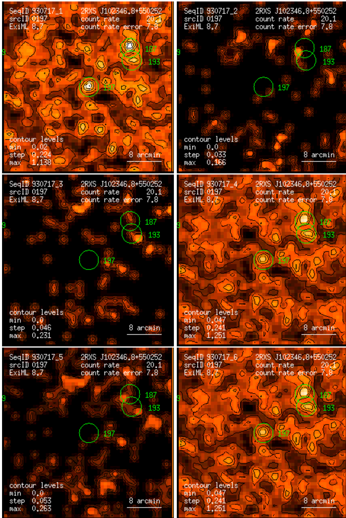
Figure 197: RASS 930717: detection 0197: band rate images, Gaussian filter: (1) PSPC channels 11 – 41, (2) 52 – 90, (3) 91 – 201, (4) 11 – 235, (5) 52 – 201, (6) 11 – 201. Broad band rates in counts/ks. Band rate contour levels in counts/ks/arcmin 2 .
