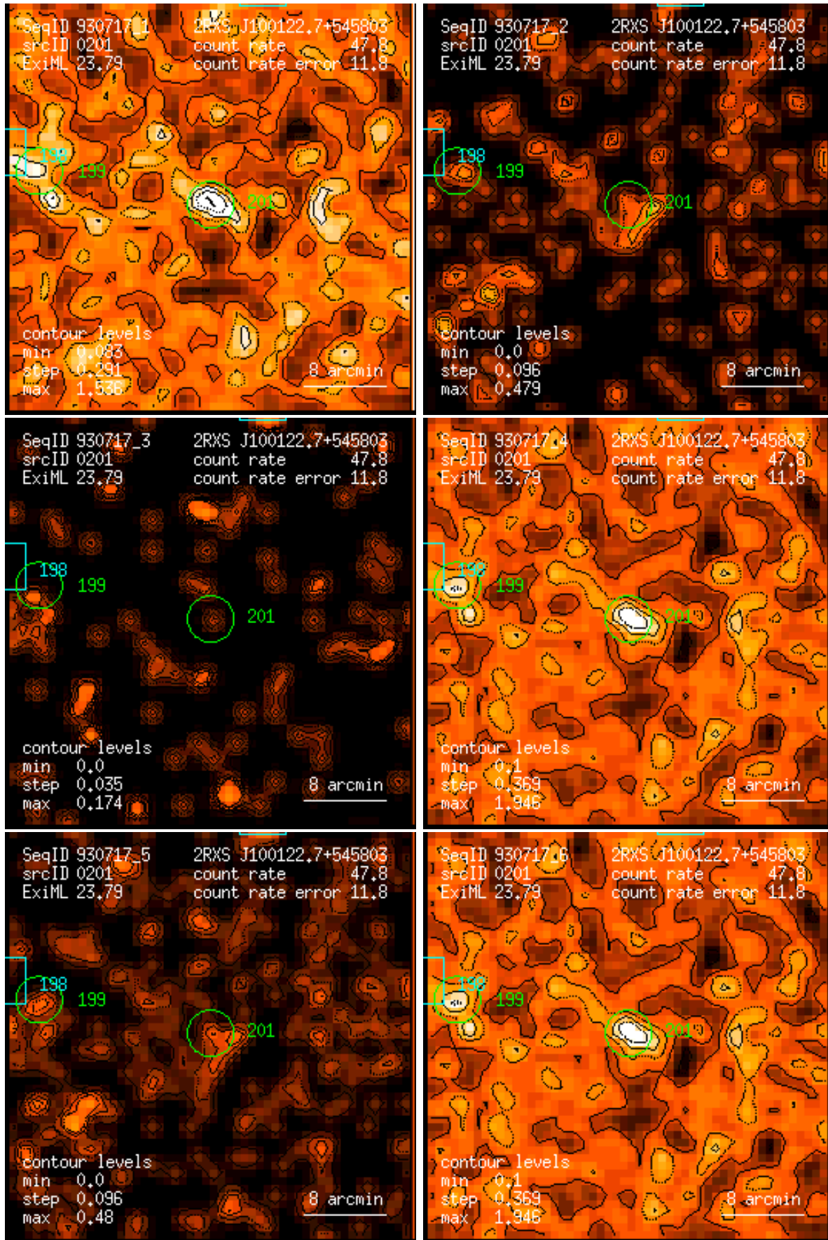
Figure 201: RASS 930717: detection 0201: band rate images, Gaussian filter: (1) PSPC channels 11 – 41, (2) 52 – 90, (3) 91 – 201, (4) 11 – 235, (5) 52 – 201, (6) 11 – 201. Broad band rates in counts/ks. Band rate contour levels in counts/ks/arcmin 2 .
