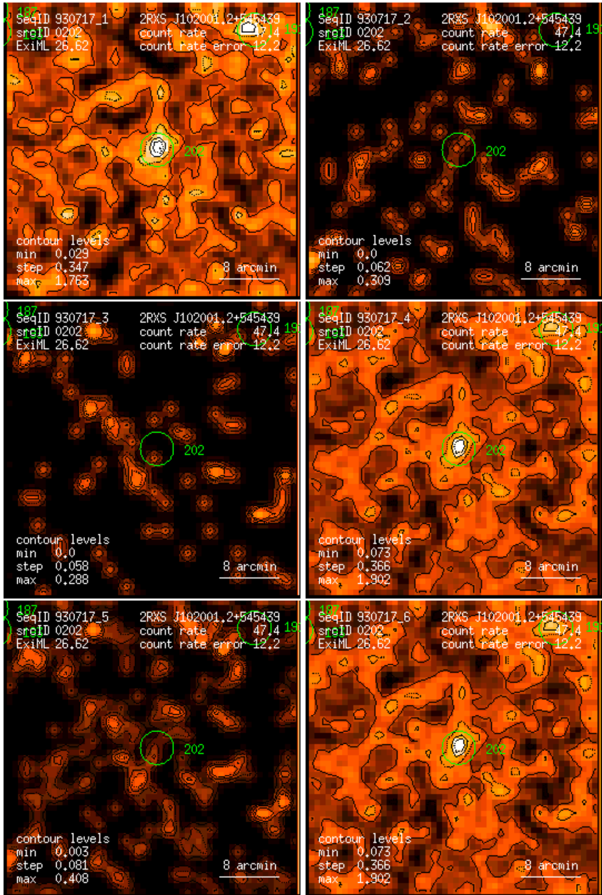
Figure 202: RASS 930717: detection 0202: band rate images, Gaussian filter: (1) PSPC channels 11 – 41, (2) 52 – 90, (3) 91 – 201, (4) 11 – 235, (5) 52 – 201, (6) 11 – 201. Broad band rates in counts/ks. Band rate contour levels in counts/ks/arcmin 2 .
