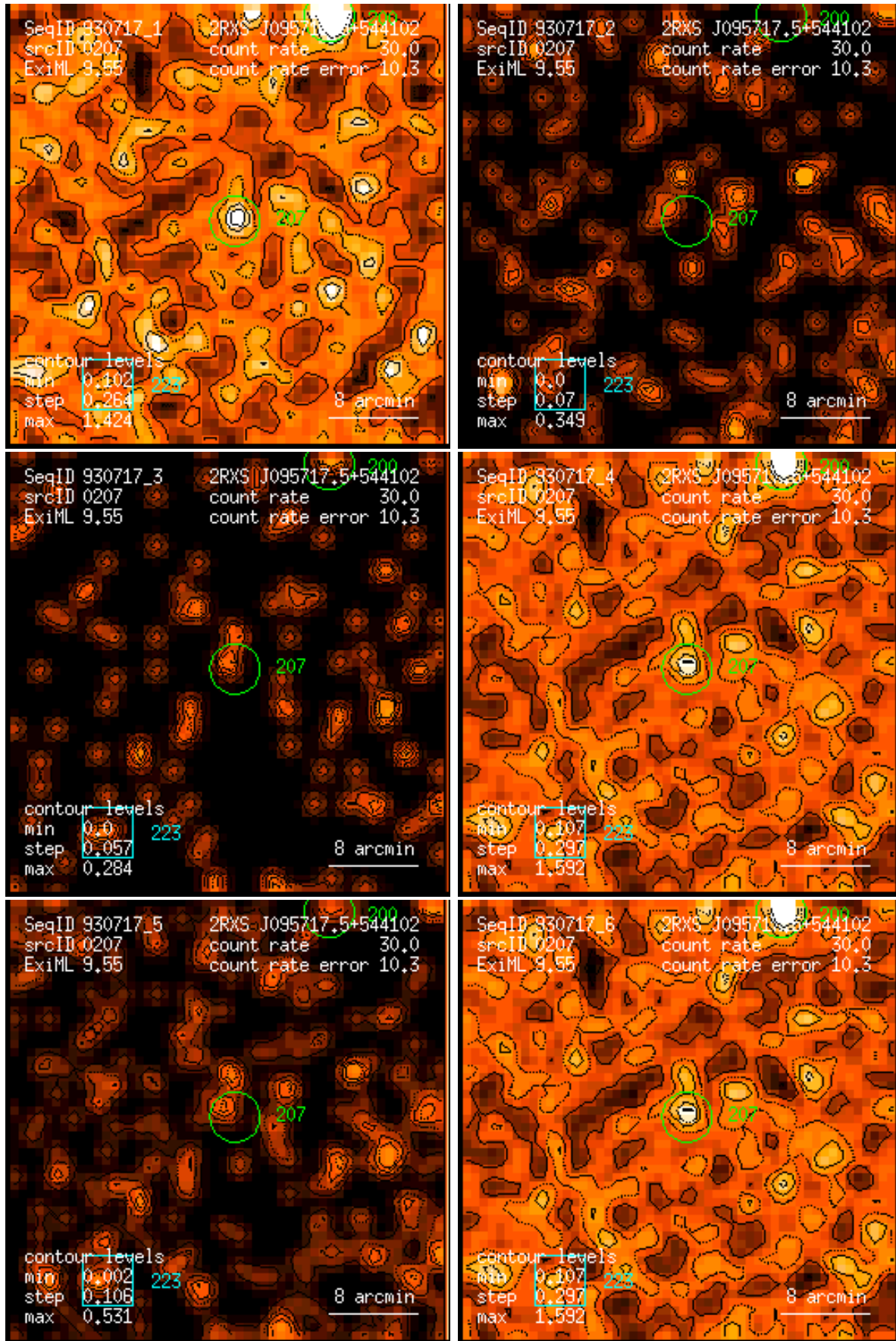
Figure 207: RASS 930717: detection 0207: band rate images, Gaussian filter: (1) PSPC channels 11 – 41, (2) 52 – 90, (3) 91 – 201, (4) 11 – 235, (5) 52 – 201, (6) 11 – 201. Broad band rates in counts/ks. Band rate contour levels in counts/ks/arcmin 2 .
