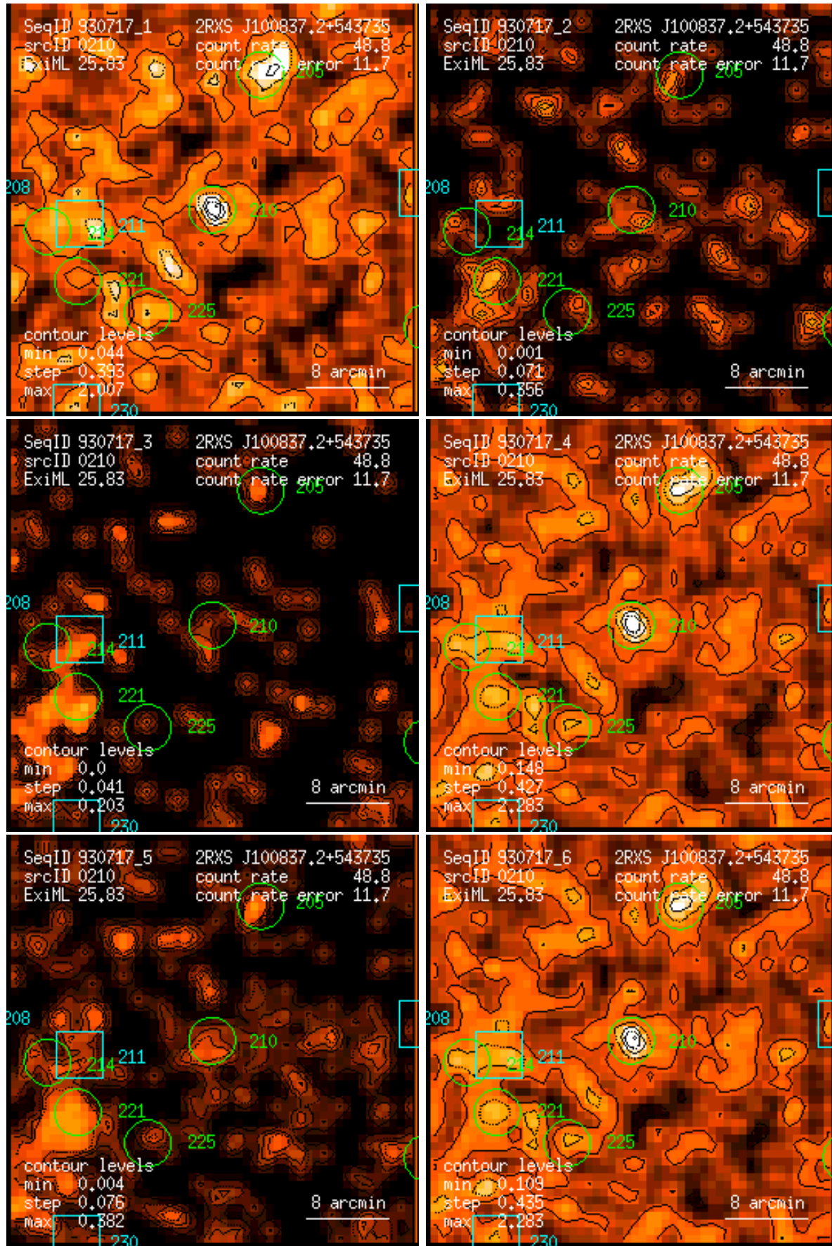
Figure 210: RASS 930717: detection 0210: band rate images, Gaussian filter: (1) PSPC channels 11 – 41, (2) 52 – 90, (3) 91 – 201, (4) 11 – 235, (5) 52 – 201, (6) 11 – 201. Broad band rates in counts/ks. Band rate contour levels in counts/ks/arcmin 2 .
