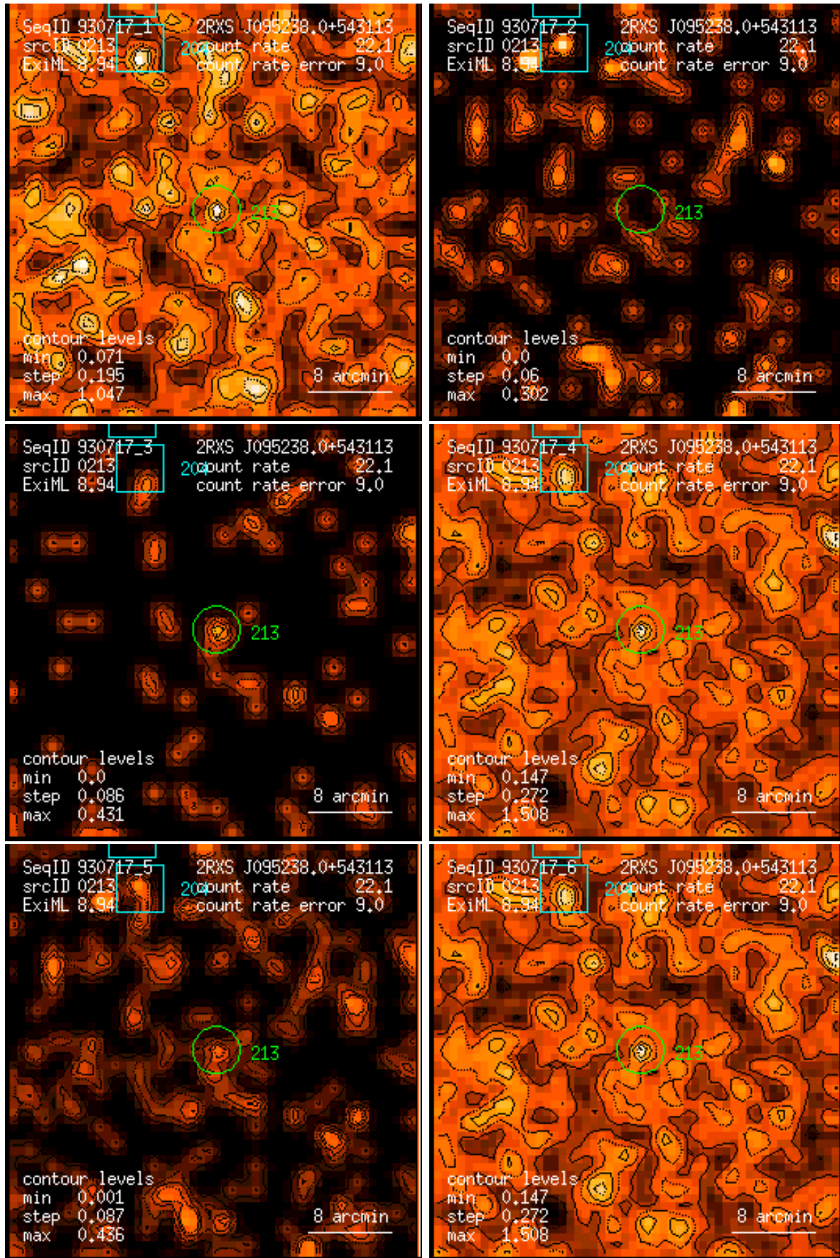
Figure 213: RASS 930717: detection 0213: band rate images, Gaussian filter: (1) PSPC channels 11 – 41, (2) 52 – 90, (3) 91 – 201, (4) 11 – 235, (5) 52 – 201, (6) 11 – 201. Broad band rates in counts/ks. Band rate contour levels in counts/ks/arcmin 2 .
