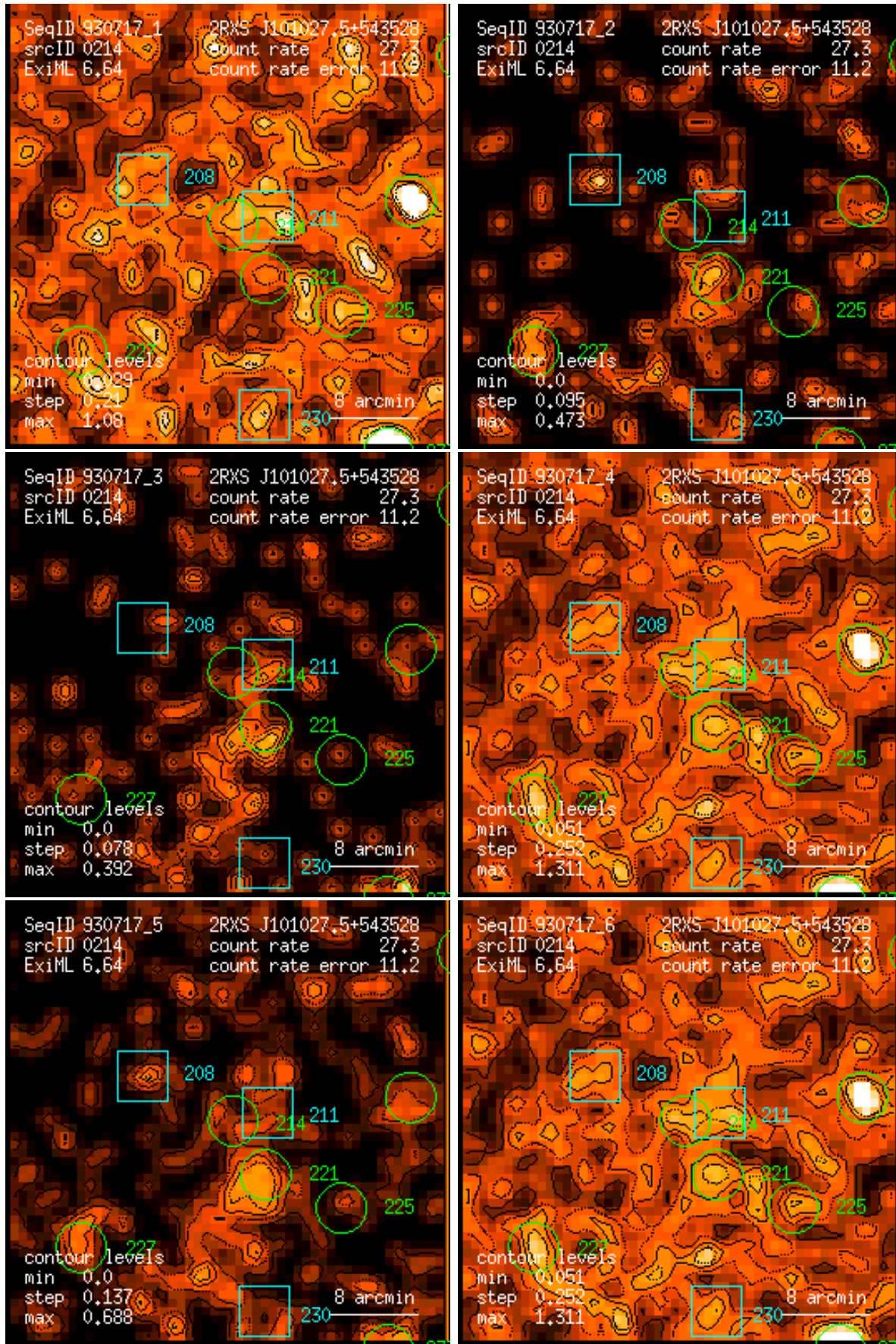
Figure 214: RASS 930717: detection 0214: band rate images, Gaussian filter: (1) PSPC channels 11 – 41, (2) 52 – 90, (3) 91 – 201, (4) 11 – 235, (5) 52 – 201, (6) 11 – 201. Broad band rates in counts/ks. Band rate contour levels in counts/ks/arcmin 2 .
