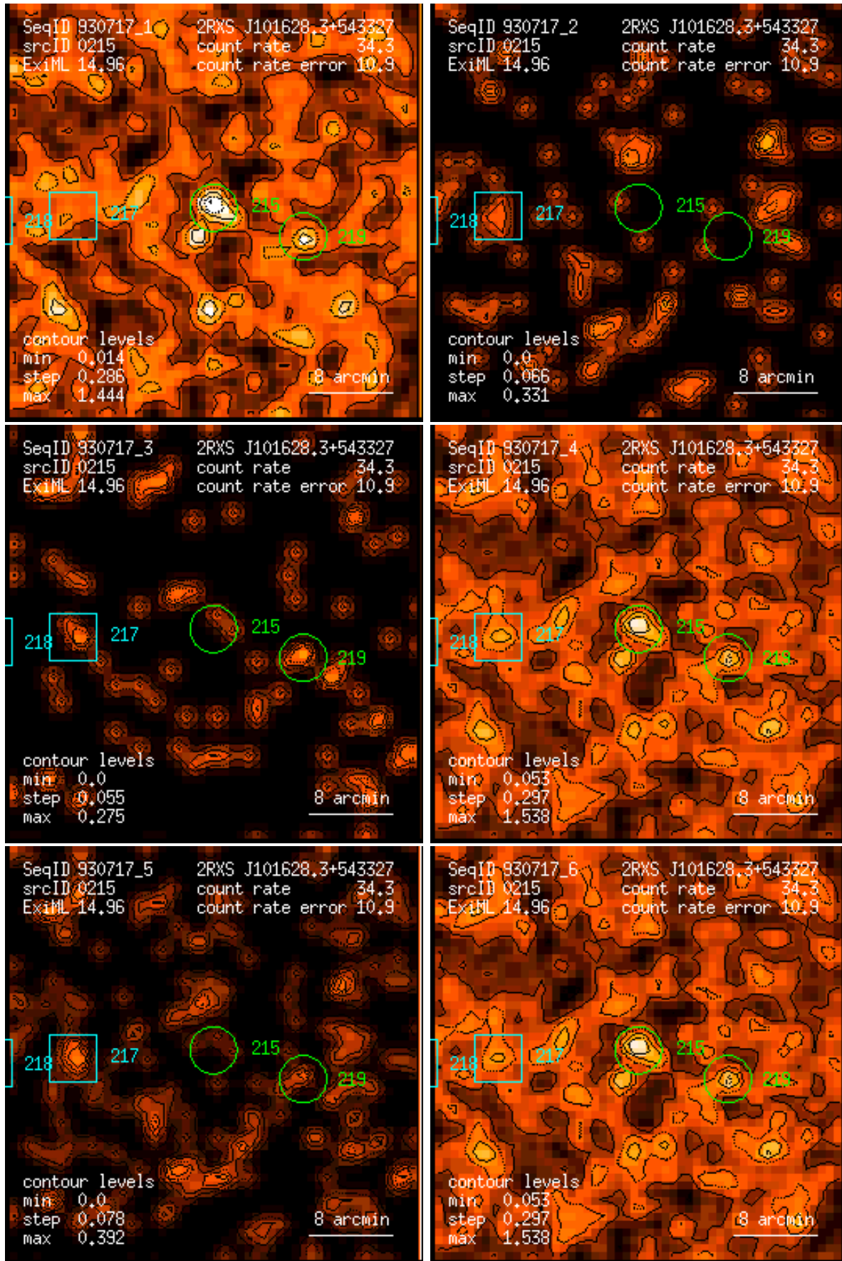
Figure 215: RASS 930717: detection 0215: band rate images, Gaussian filter: (1) PSPC channels 11 – 41, (2) 52 – 90, (3) 91 – 201, (4) 11 – 235, (5) 52 – 201, (6) 11 – 201. Broad band rates in counts/ks. Band rate contour levels in counts/ks/arcmin 2 .
