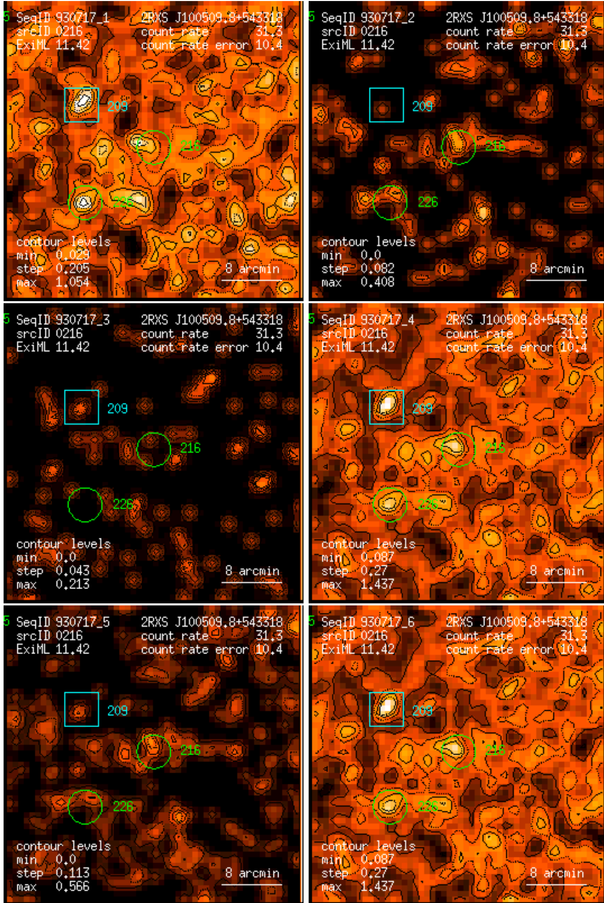
Figure 216: RASS 930717: detection 0216: band rate images, Gaussian filter: (1) PSPC channels 11 – 41, (2) 52 – 90, (3) 91 – 201, (4) 11 – 235, (5) 52 – 201, (6) 11 – 201. Broad band rates in counts/ks. Band rate contour levels in counts/ks/arcmin 2 .
