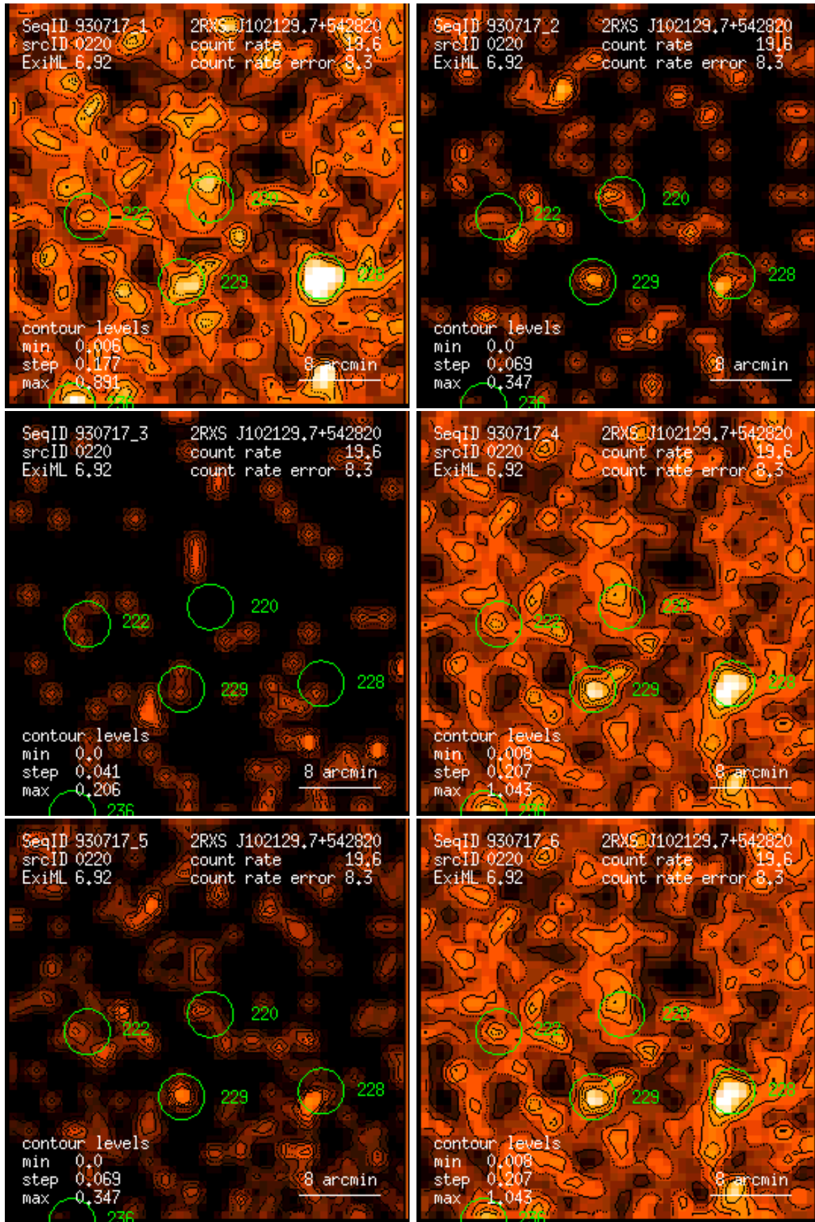
Figure 220: RASS 930717: detection 0220: band rate images, Gaussian filter: (1) PSPC channels 11 – 41, (2) 52 – 90, (3) 91 – 201, (4) 11 – 235, (5) 52 – 201, (6) 11 – 201. Broad band rates in counts/ks. Band rate contour levels in counts/ks/arcmin 2 .
